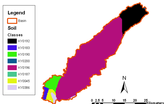
Fig. 3. Nyangores sub-basin soil types (FAO Soil database).
