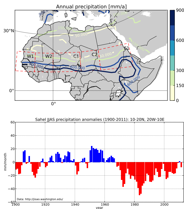
Fig. 1. Annual mean precipitation [ \text{mm yr}^{-1} ] in the Sahelian region. Bounding boxes for regions used for detailed analysis extend between 10 and 20° N. Longitudinal extent is given as W1 (20–10° W), W2 (10–00° W), C1 (00° W–15° E), C2 (15–25° E), and E1 (25–40° E) (data: GPCP) (top panel). Sahel rainfall anomalies for the period 1900–2011 and the region from 10–20° N, 20° W–10° E (data from http://jisao.washington.edu/ , Ali and Lebel, 2009) (bottom panel).
