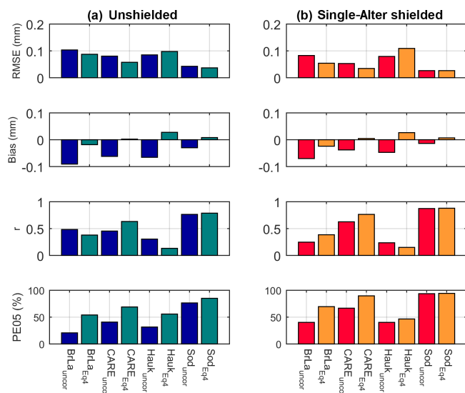
Figure 9. SLED gauge statistics for four sites, calculated from the difference between the DFAR precipitation and both the uncorrected (dark blue for (a) unshielded and red for (b) single-Alter shielded) and the adjusted (light blue for (a) unshielded and orange for (b) single-Alter shielded) precipitation using Eq. (4). The RMSE, mean bias, correlation coefficient ( r ), and the percent of events within 0.05 mm range (PE05 mm) of the reference are shown for the individual sites.
