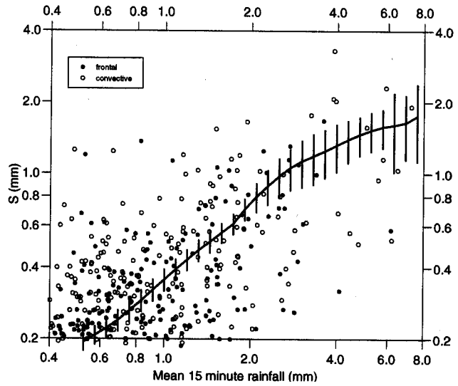
Fig. 8. Standard error, S , of rainfall estimate from a single gauge as a function of total rainfall in a 15 minute interval over the low relief square. Vertical lines indicate the 90% range in sampling uncertainty and the symbols \bullet and \circ denote frontal and convective rainfall types respectively.
