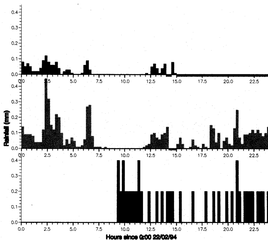
Fig. 5. Data quality control during unusual events using radar and raingauge hyetographs: snowfall event on 22 February 1994 as measured by the Cobacombe and Wardon Hill radars and by the raingauge at Bridge Farm, which records only as snow starts to melt in the funnel.
