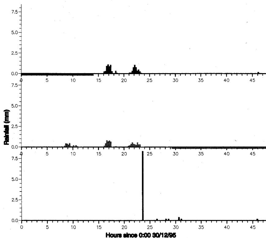
Fig. 6. Data quality control during unusual events using radar and raingauge hyetographs: freezing rain event late in the evening of 30 December 1995 as measured by the Cobacombe and Wardon Hill radars and by the raingauge at Bridge Farm, giving an anomalous spike.
