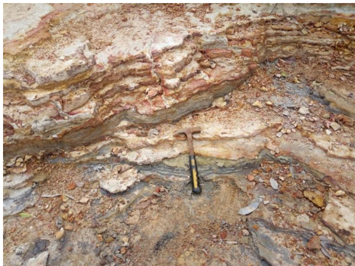
Figure 27: Laminated heterolytic unit
