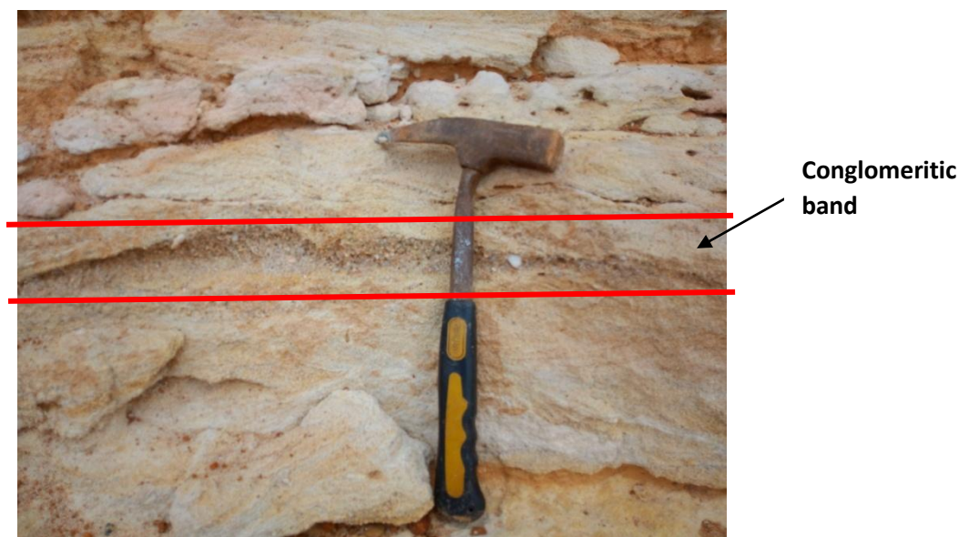
Figure 5: Conglomeritic band as seen in Amaozara sand mine.
