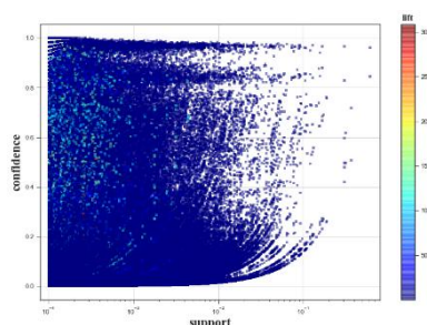
Figure 6. Confidence-Support relationship with the colors representing relevant LIFT values
