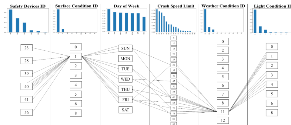
Figure8. Illustration of frequent itemsets with higher Support for each Safety Device
