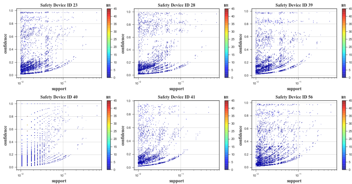
Figure 7. Support-confidence relation of each safety device
