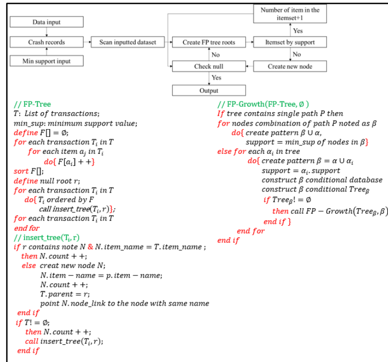
Figure 4. The flow chart and pseudo-code of the FP-Growth algorithm [25]
