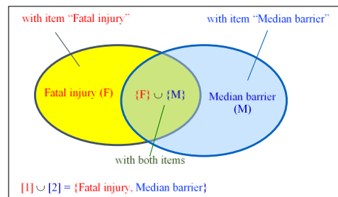
Figure 2. A subtle notation of itemset “ X = \text{Fatal injury} \cup Y = \text{Median barrier} ”, which is motivated from [8]
