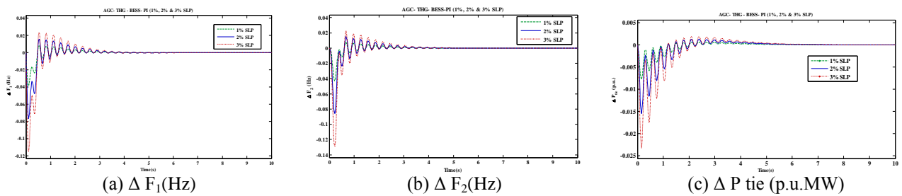
Fig 4. Simulation results of BESS with two-Area Thermal, Hydro and Gas Plant (THG) System with PI Controller for Power System with (1%, 2% & 3% SLP).
