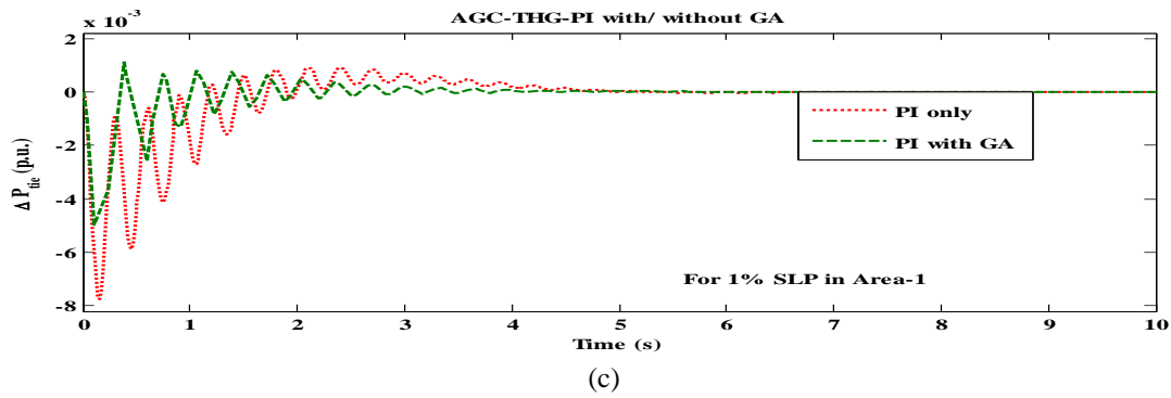
Fig 5(a, b, c) AGC- THG- PI with/ without GA for 1% SLP in Area -1
