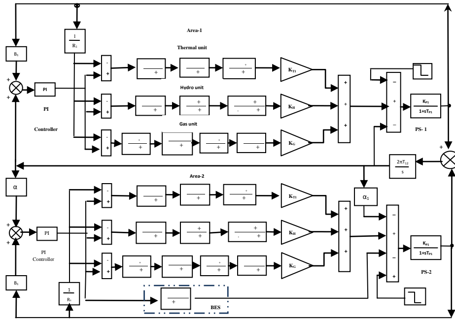
Fig1. Battery Energy Storage System with model of Two-Area (THG) System with PI Controller for Power System
