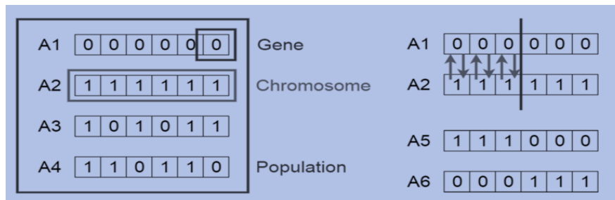
Fig2. Genetic algorithm
