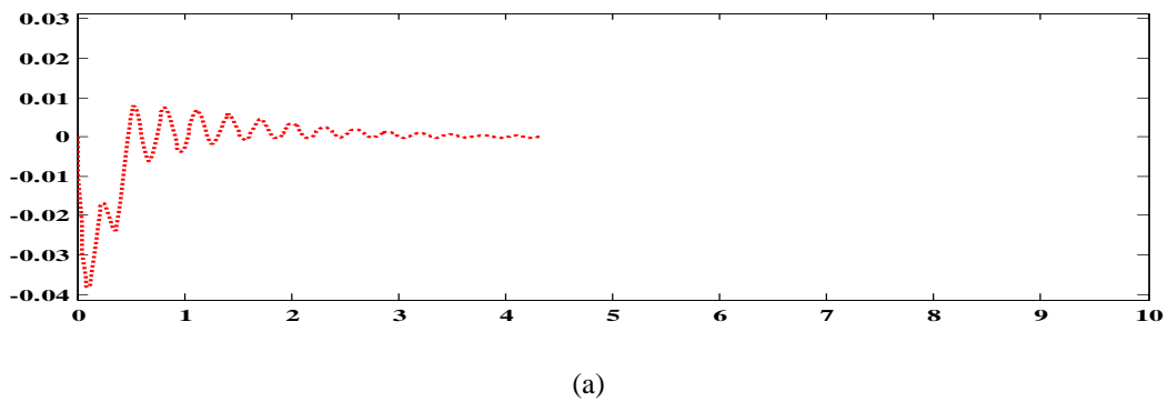
Fig 5(a, b, c) AGC- THG- PI with/ without GA for 1% SLP in Area -1
