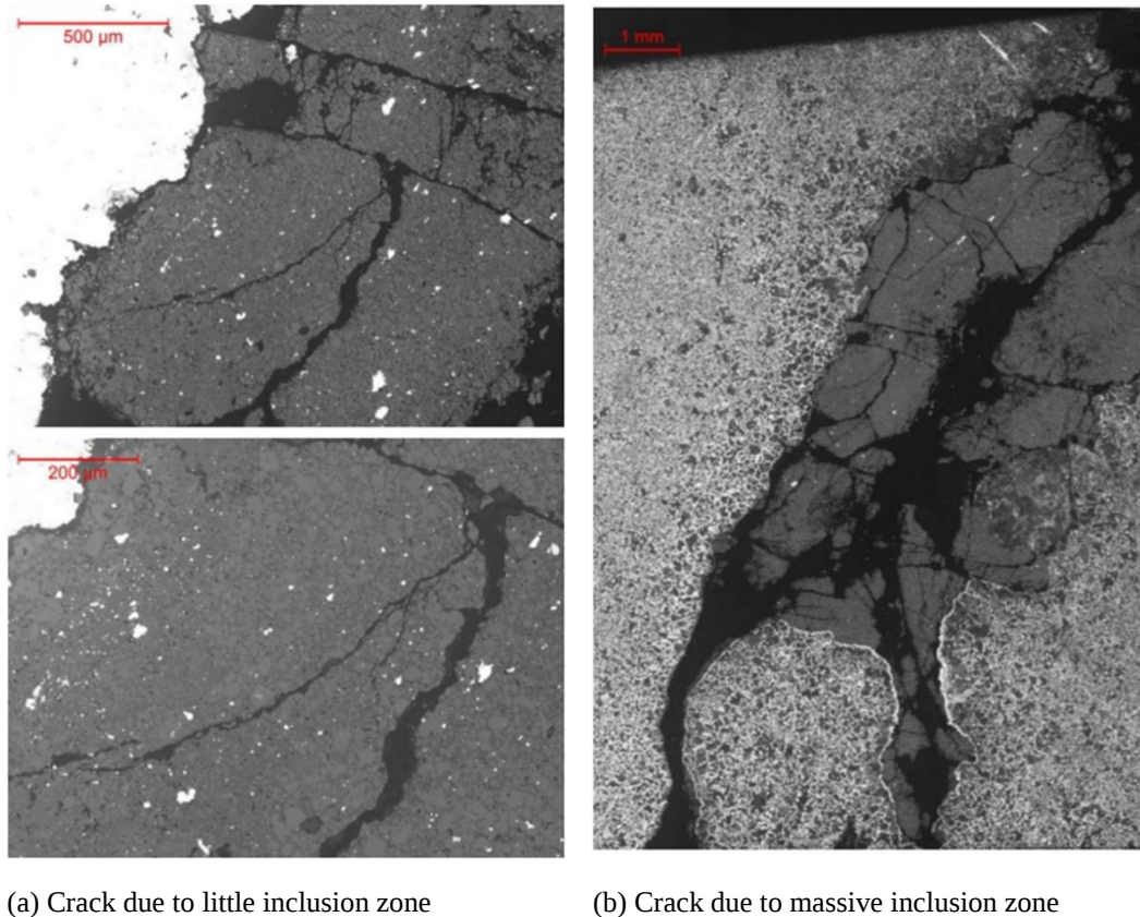
Figure 10. Crack zone image of SMS surface by the optical microscope after forging
