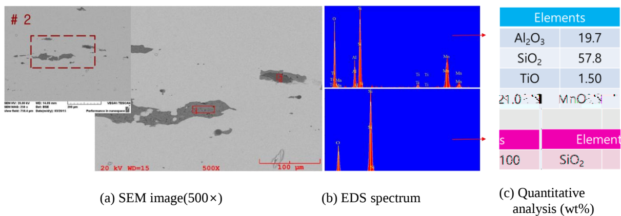
Figure 5. SEM image and EDS analysis of the flaws on FCS #2
