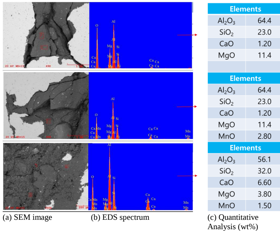
Figure 6. SEM image and EDS analysis of the flaws on SMS
