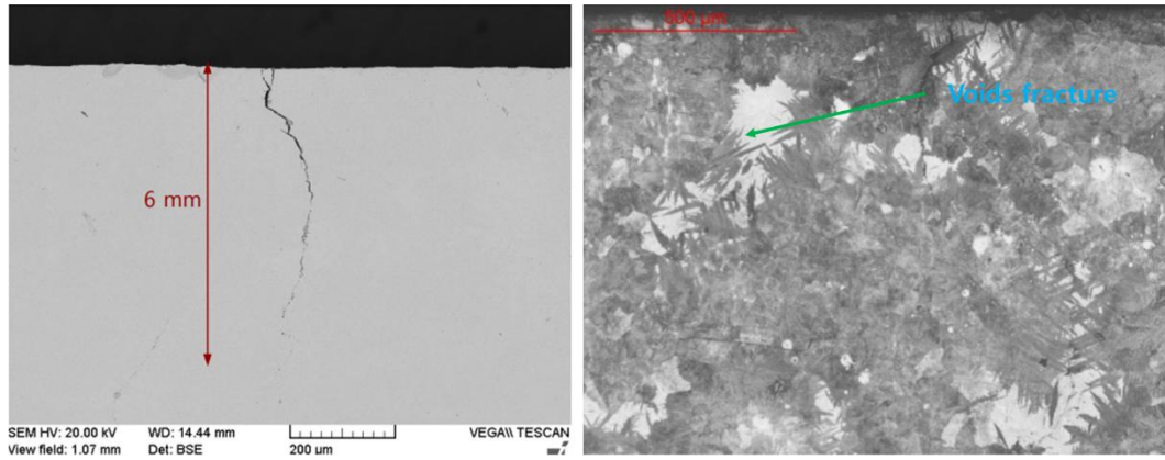
(a) Vertical crack depth from surface (b) Voids fracture image against crack direction
