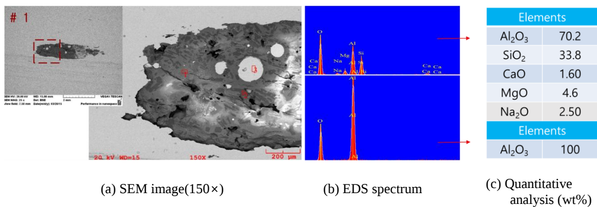
Figure 4. SEM image and EDS analysis of the flaws on FCS #1
