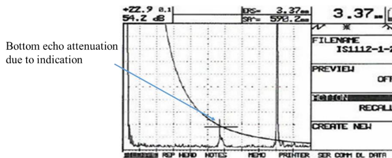
Figure 3. Defect indication pattern by sedimentary crystallization zone in the FCS : Inclusion trap pattern
