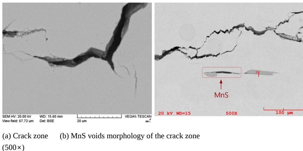
Figure 7. SEM images of the crack fracture zone on NCMS after forging
