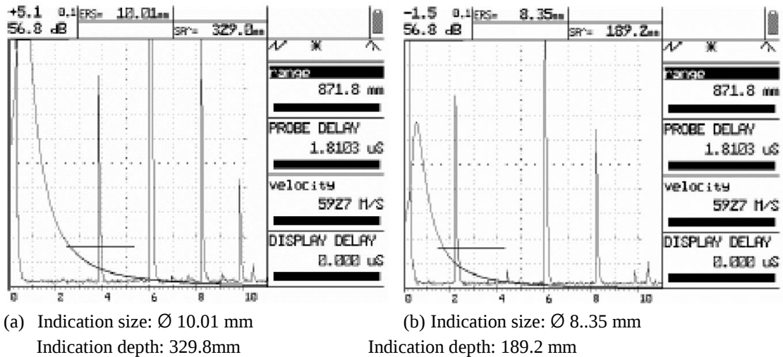
Figure 2. Defects indication pattern by V-type segregation zone in the center of the FCS
