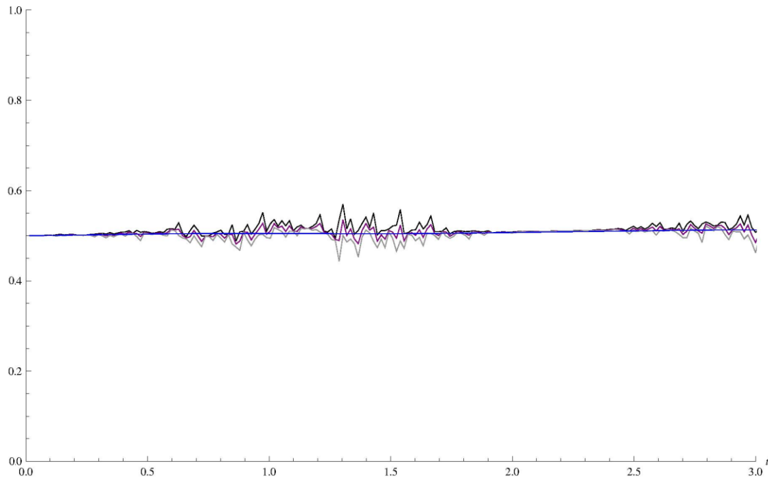
Fig. 1. Dynamic behavior of the stochastic bounds and the Ermakov invariant with t \in [0, \pi] , the gray color corresponds to the m = 0 additive noise of amplitude \alpha_\Omega = 0.15 , lower bound, the magenta color corresponds to the amplitude \alpha_\Omega = 0.1 and the black color corresponds to the amplitude \alpha_\Omega = 0.2 (upper bound).
