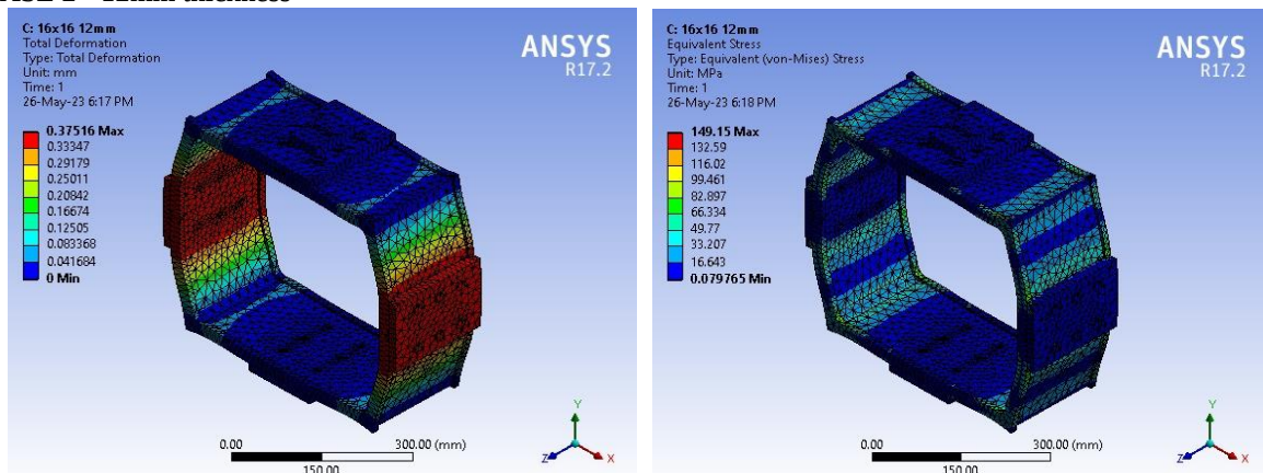
Figure 9:The stress analysis and total deformation images are shown above for 16x16-inch box with an 12-mm wall thickness
