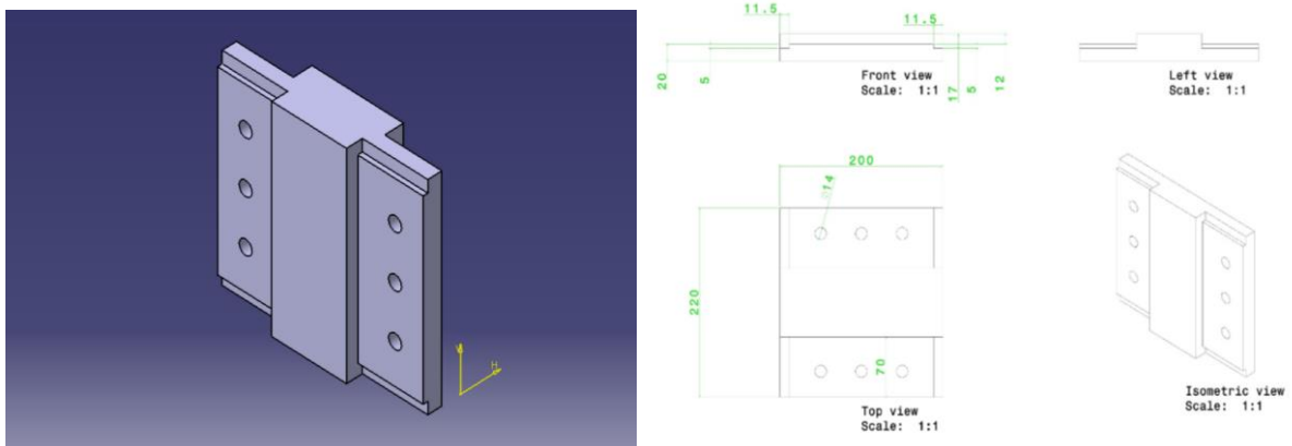
Figure 3: 19 inches * 19 inches Side plate
