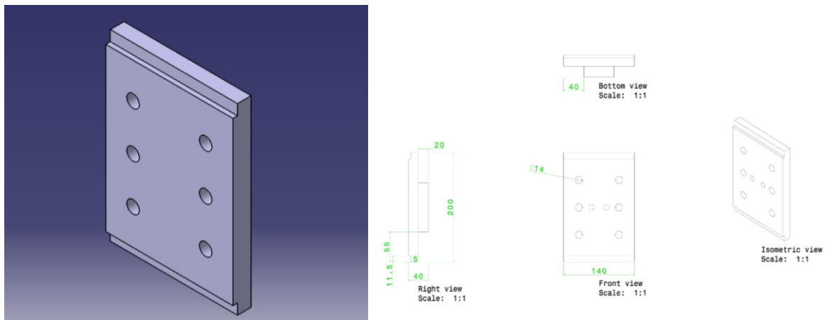
Figure 2 :16 inches * 16 inches Side plate
