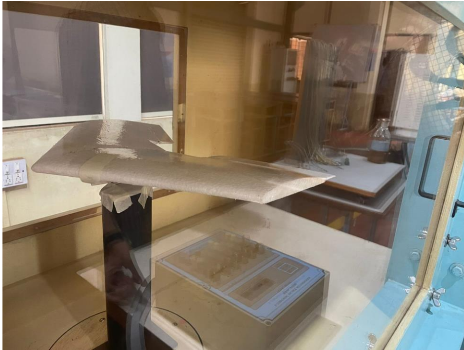
figure 7.1.1. model placed in wind tunnel
