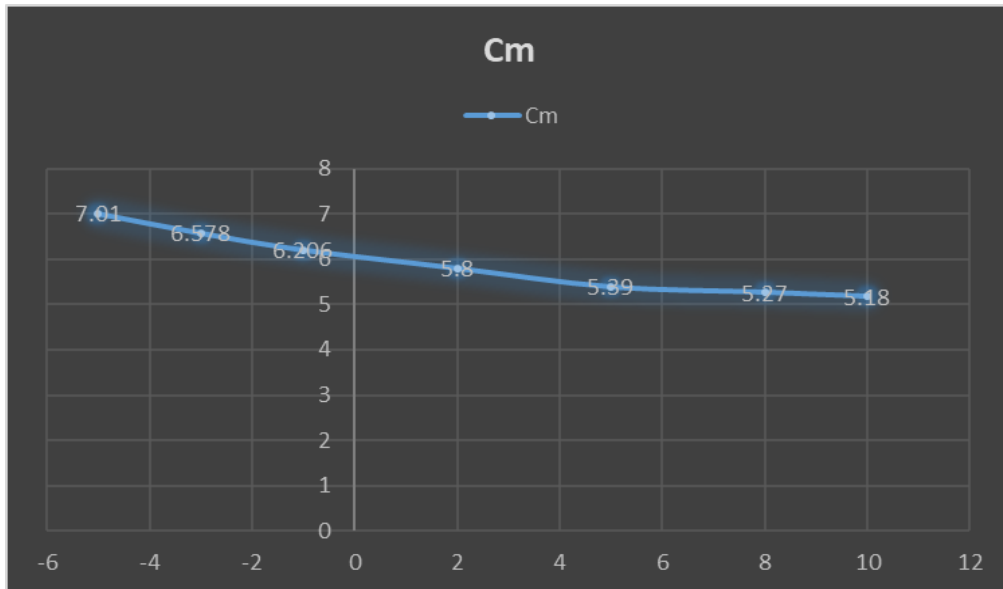
figure 7.4.1 graph Cm v/s α
