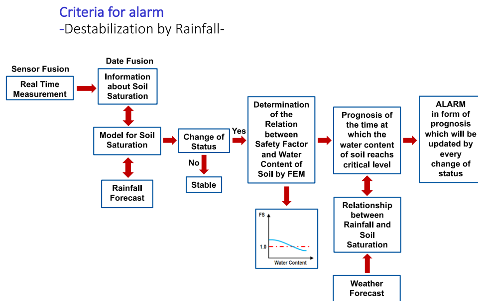
Figure 3: Flow chart of the process for the evaluation of the safety status of landslides in destabilization mechanism by rainfall.
