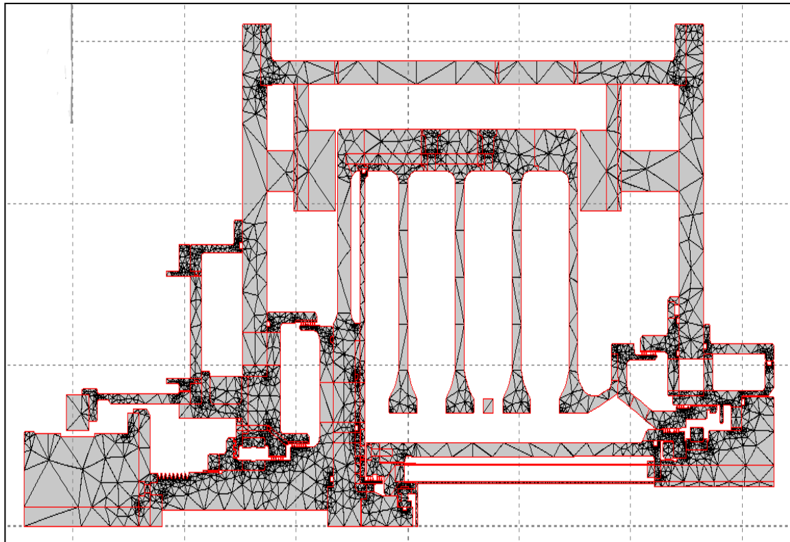
Figure 2.1: The geometry of the multiple cavity rig model meshed with six-node triangular elements in 2D.
