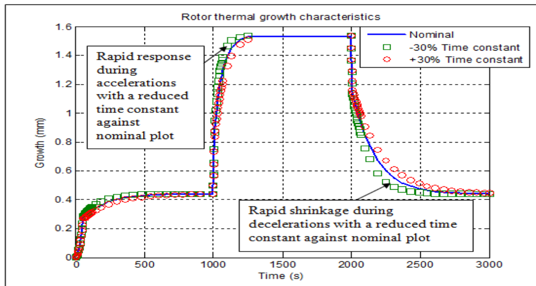
Figure 3.1: The variation of rotor tip thermal growth with time over a square cycle of stage 1 HP compressor for RB211-524 engine with (+/-30%) time constant ( \tau ) during transient operation.
