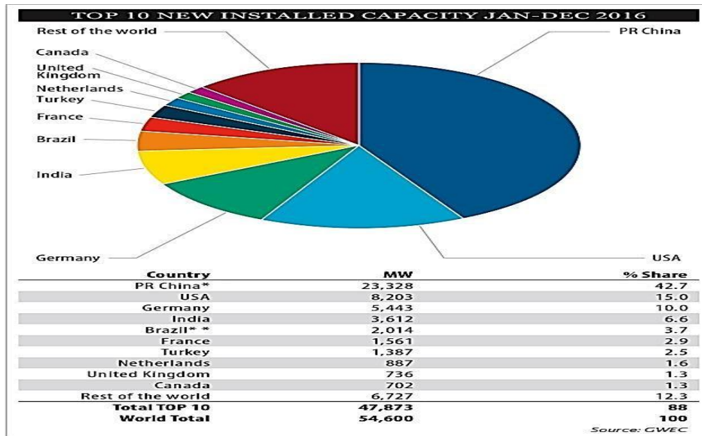
Fig.1. Installed wind capacity (2016) of world.
