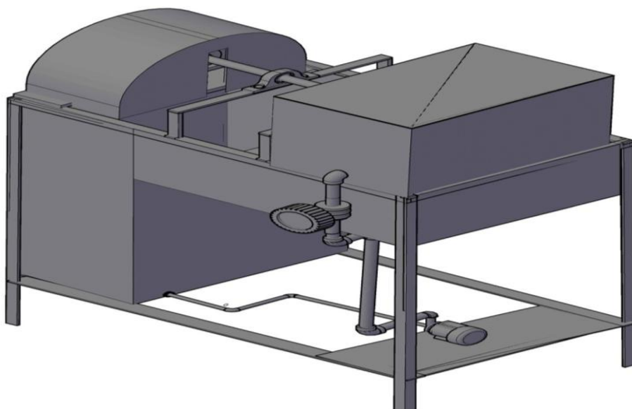
Figure 3.2: (3-D) Isometric drawing of the Front view of the Pelton wheel impulse turbine
