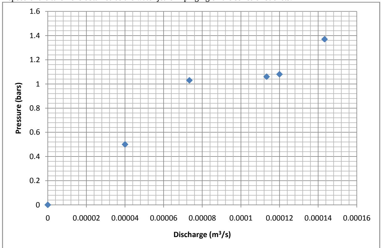
Figure 4.1: Shows the effect of Nozzle diameter on the Pressure of the turbine
