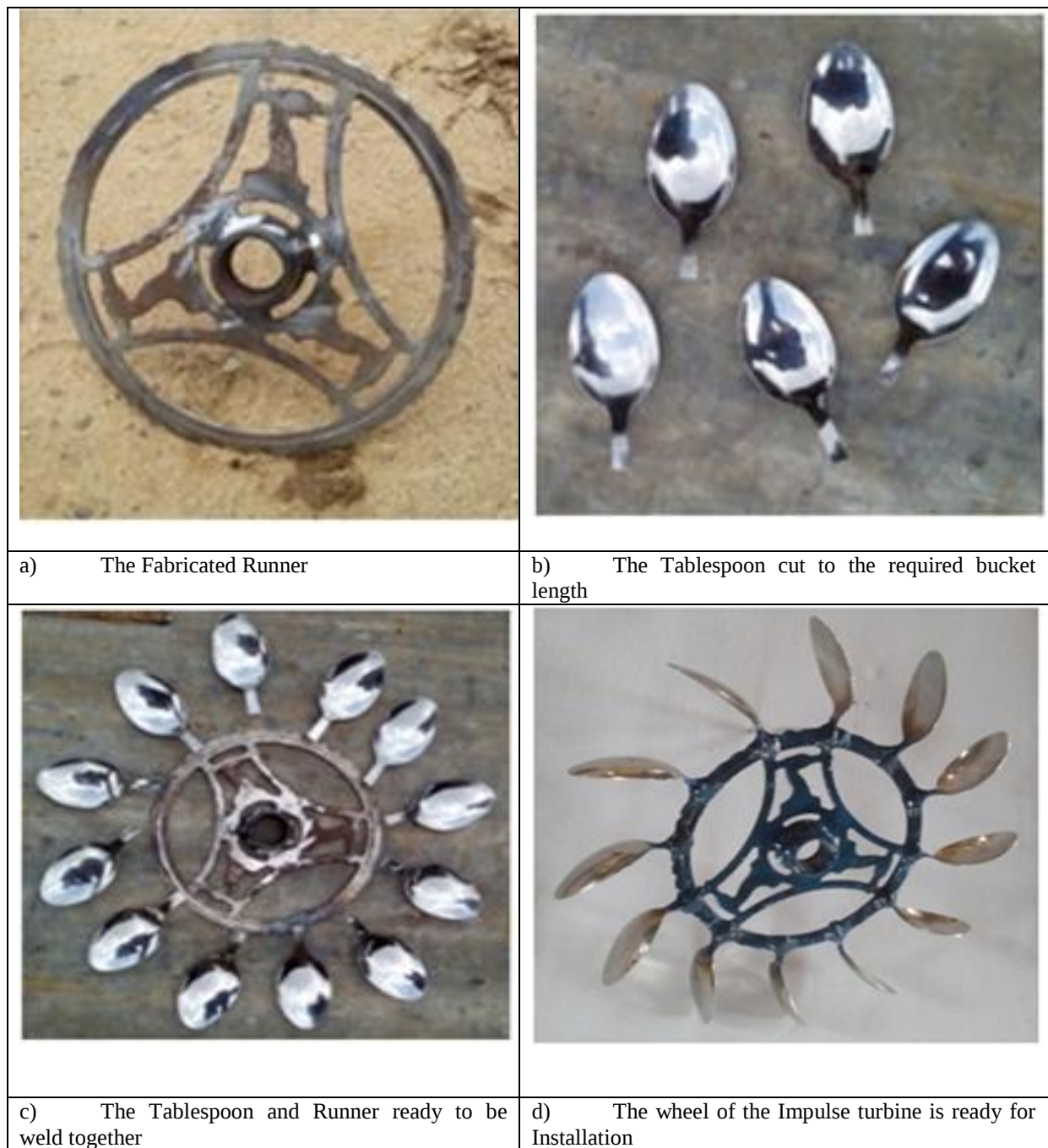
Figure 3.3: Fabrication of the Runner and the Tablespoon buckets
