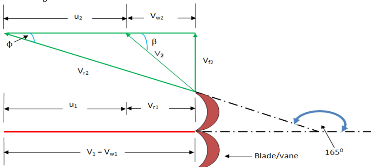
Figure 4.5: Velocity triangle diagram for the analysis of the performance of the Tablespoon Buckets Impulse Turbine
