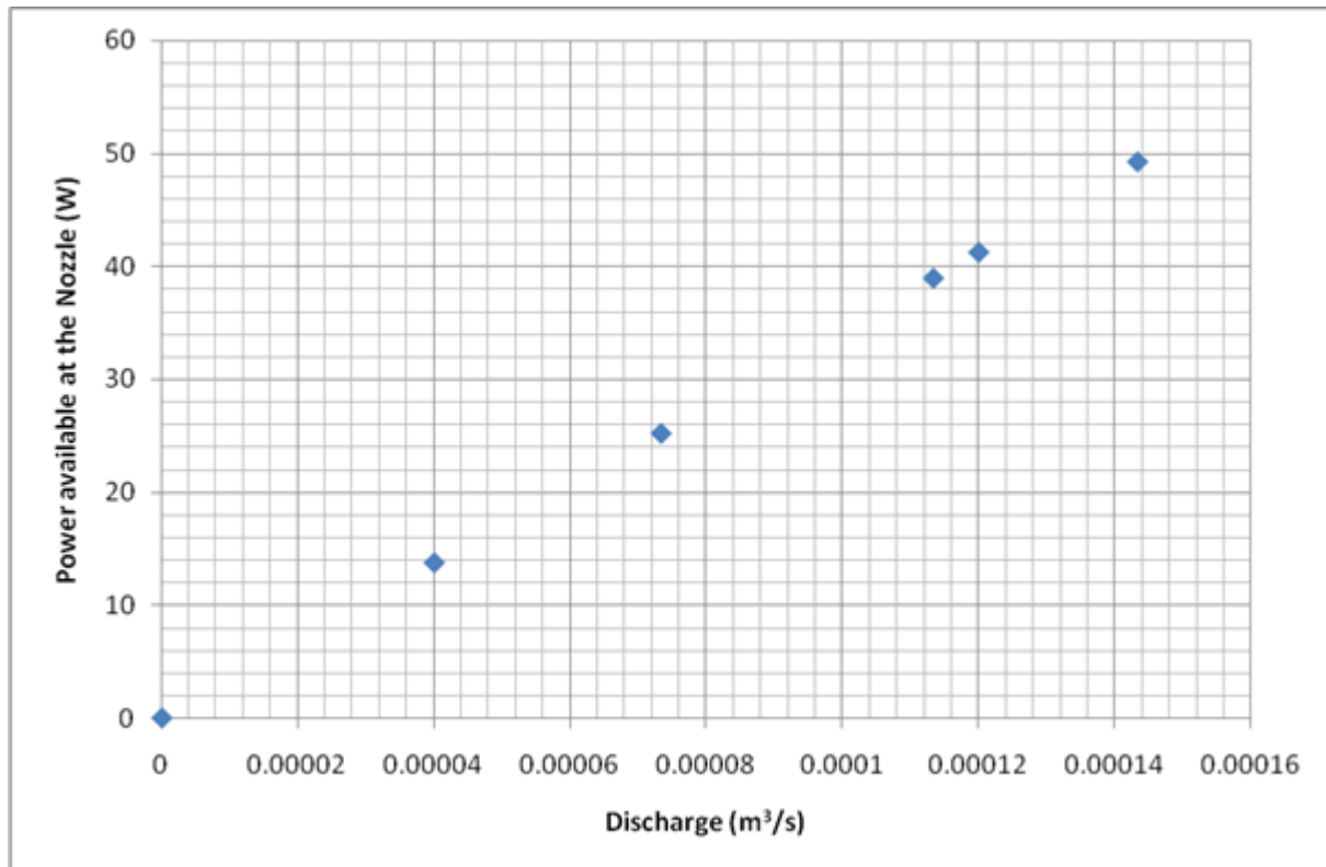
Figure: 4.4: Graph of Power available at the nozzle against Discharge of the turbine
