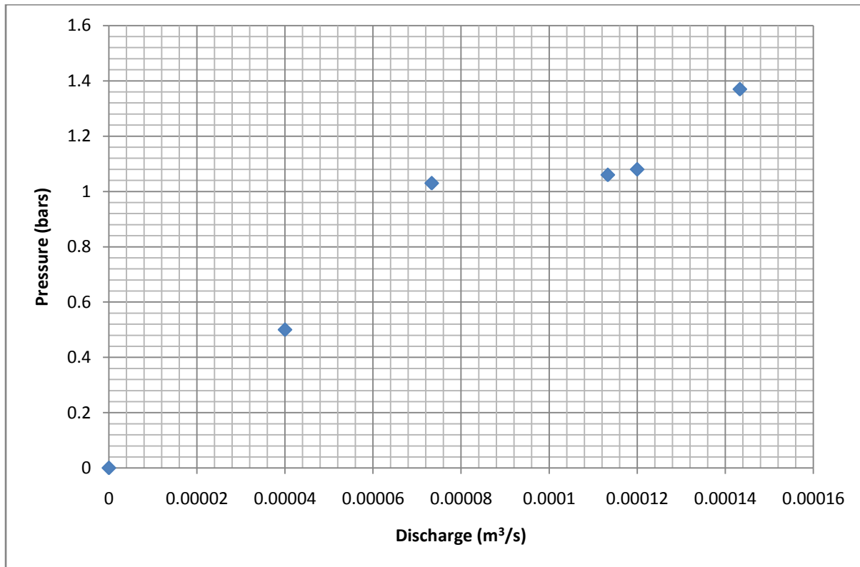
Figure 4.3: Shows the variation of Pressure with the Discharge of the Tablespoon Pelton wheel turbine
