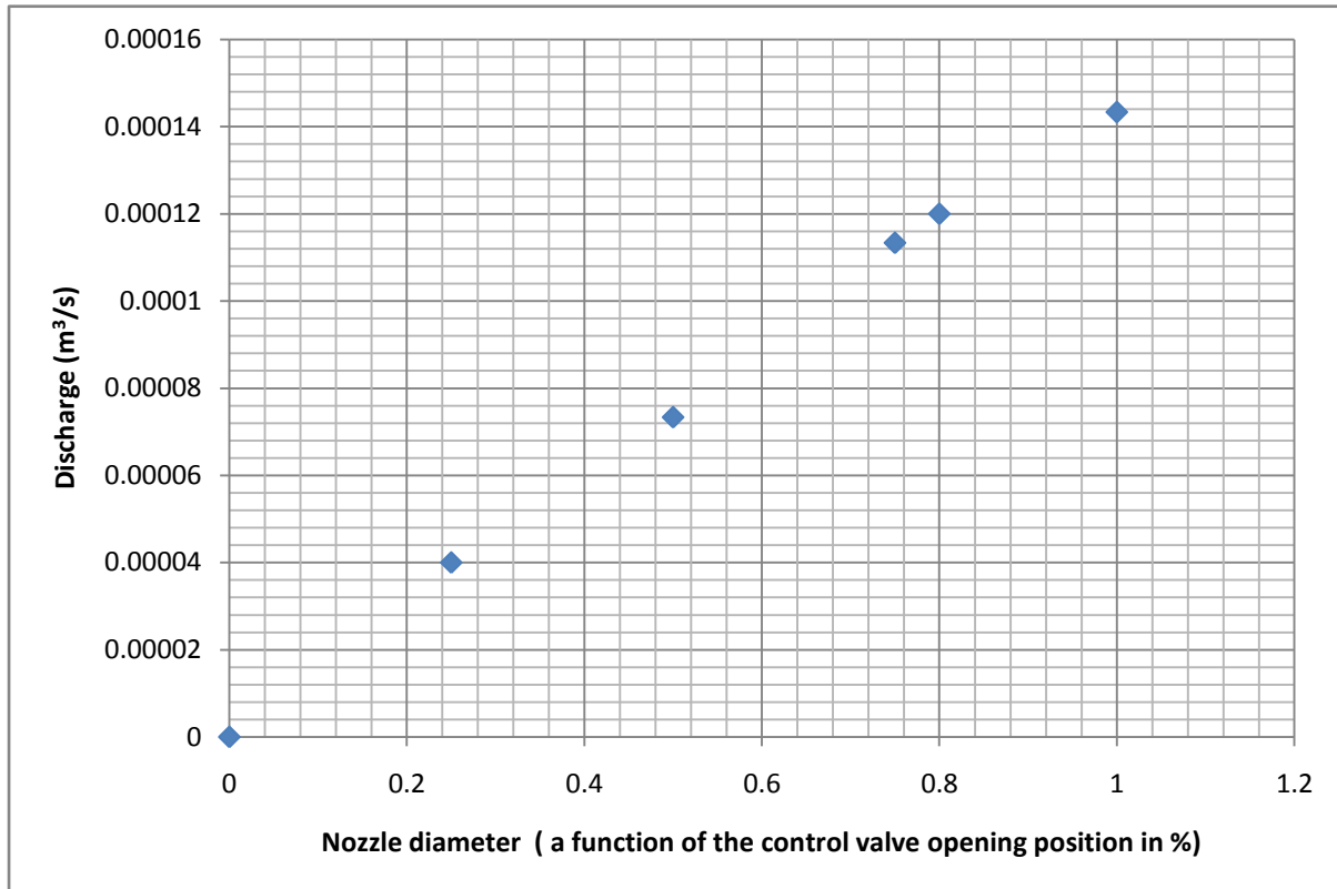
Figure 4.2: Shows the effect of Nozzle diameter on the Discharge of the turbine
