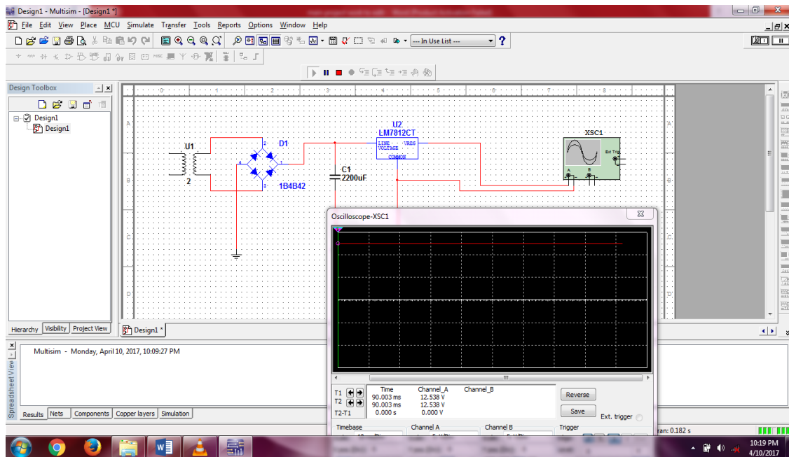
Figure 7 Signal waveform of power supply circuit
