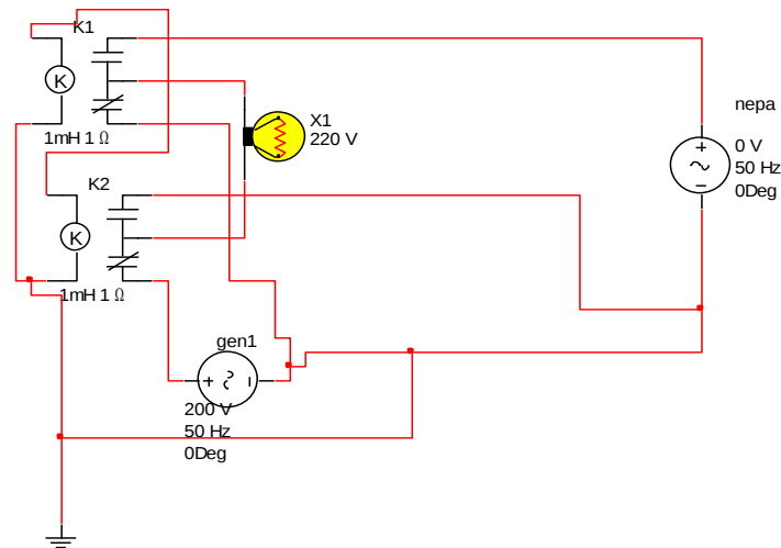
Figure 3 Changeover switch
