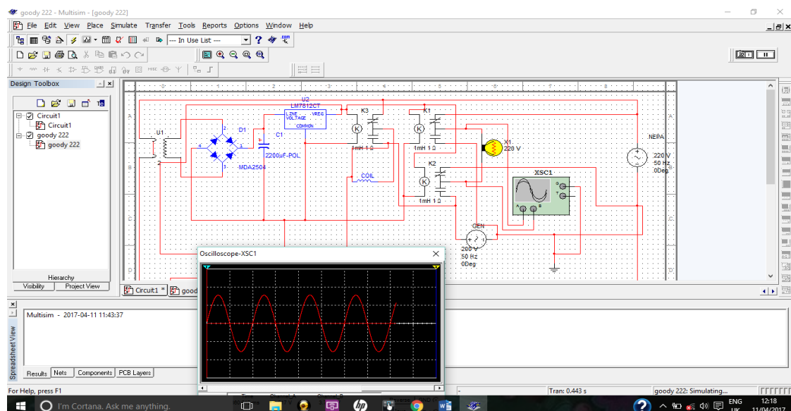
Figure 8 Signal waveform of the connected load
