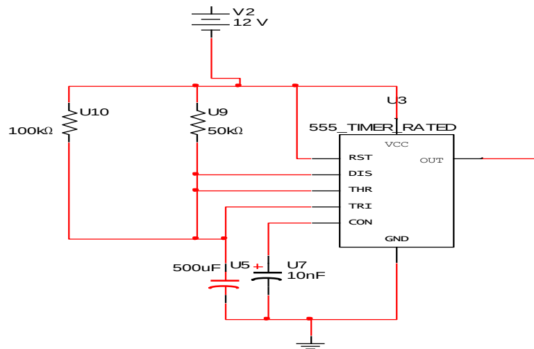
Figure. 5 The schematic diagram of the Astable 555 timer
