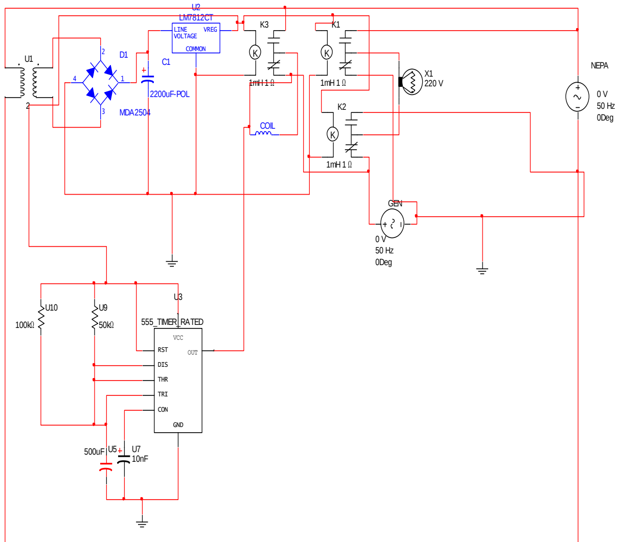
Figure6 Circuit diagram of automatic change over switch with generator trip-off mechanism
