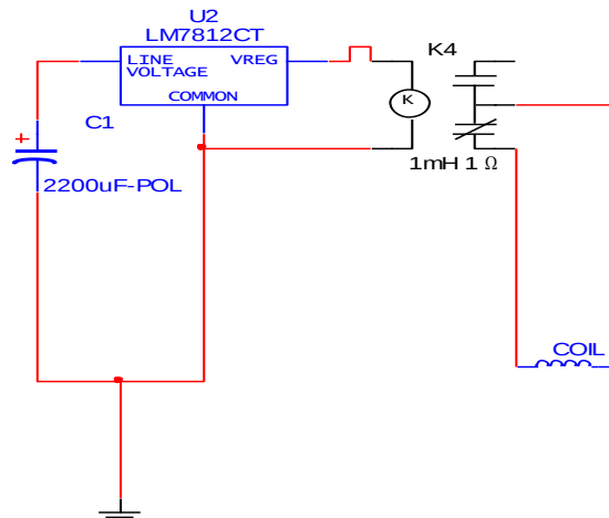
Fig. 4 Diagram of the cut-off switch
