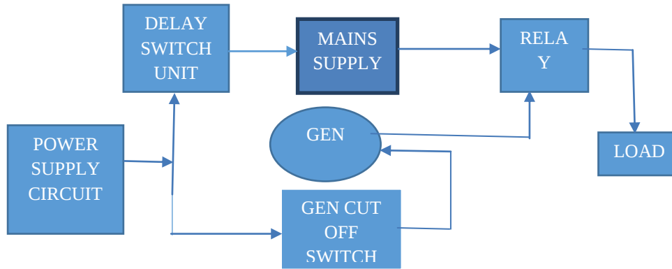
Figure 1 Conceptual Block Diagram of the proposed Automatic Change-over Switch
