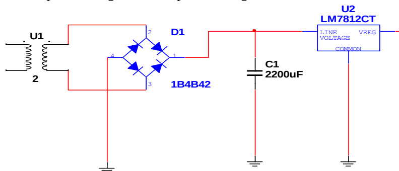
Figure 3 Power Supply Unit using Center-Tapped Transformer
