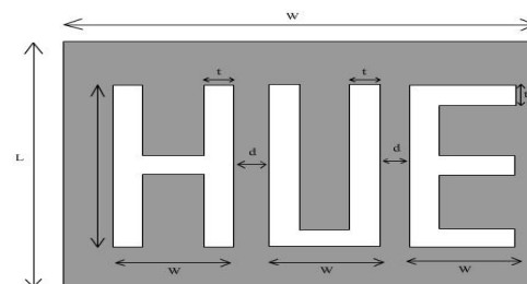
Fig. 23. Representation of HUE Slotted Microstrip Antenna
