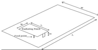
Fig. 13. Representation of planar inverted-f-antenna (PIFA)
