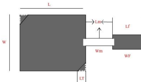
Fig. 21. Representation of wearable antenna
