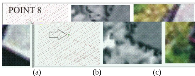
Figure 6 – (a) LIDAR cloud of points (the Point 8 is in the central area); (b) detail for the Point 8 in the intensity image; (c) detail of the Point 8 in the photographic image.
