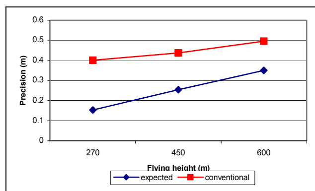
Figure 2. Effect of flying height on DEM precision
