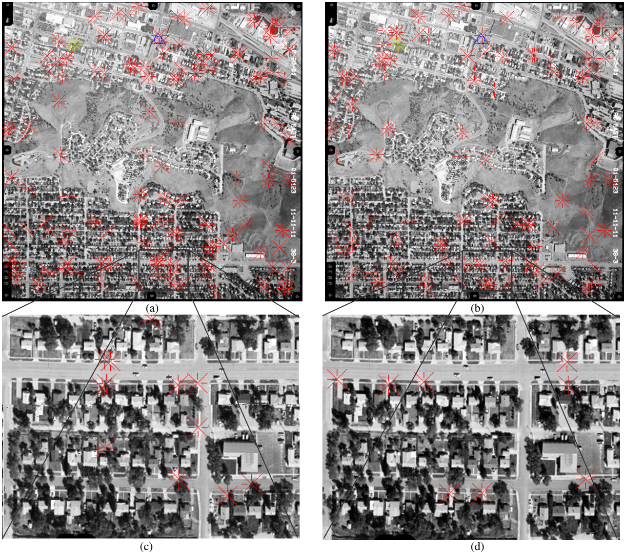
Figure 4. Automatically generated Tie/Pass Points (a), (c) extracted tie/pass points before removal of shadow points, (b), (d) extracted tie/pass points after removal of shadow points
