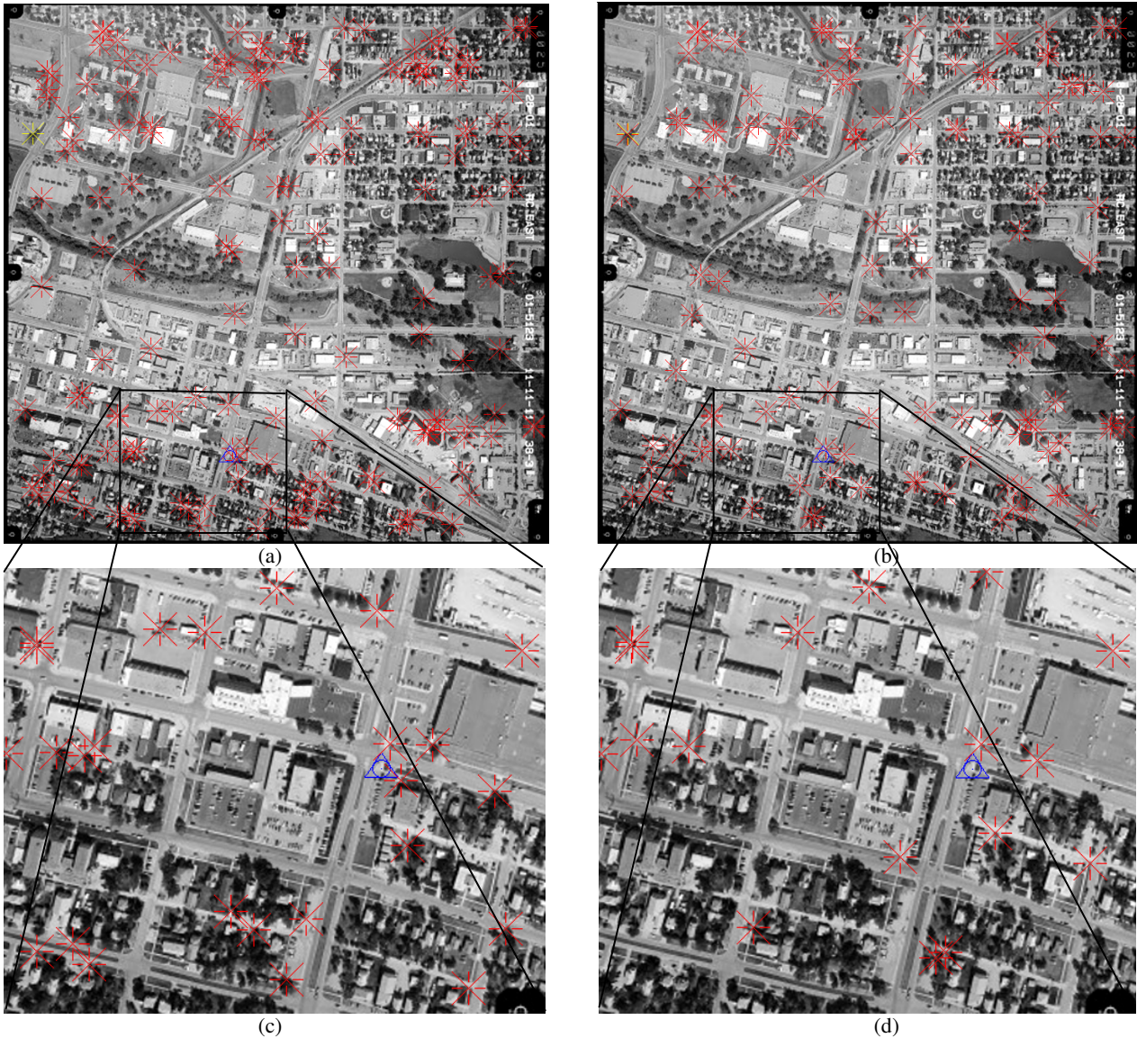
Figure 5. Automatically generated Tie/Pass Points (a), (c) extracted tie/pass points before removal of shadow points, (b), (d) extracted tie/pass points after removal of shadow points
