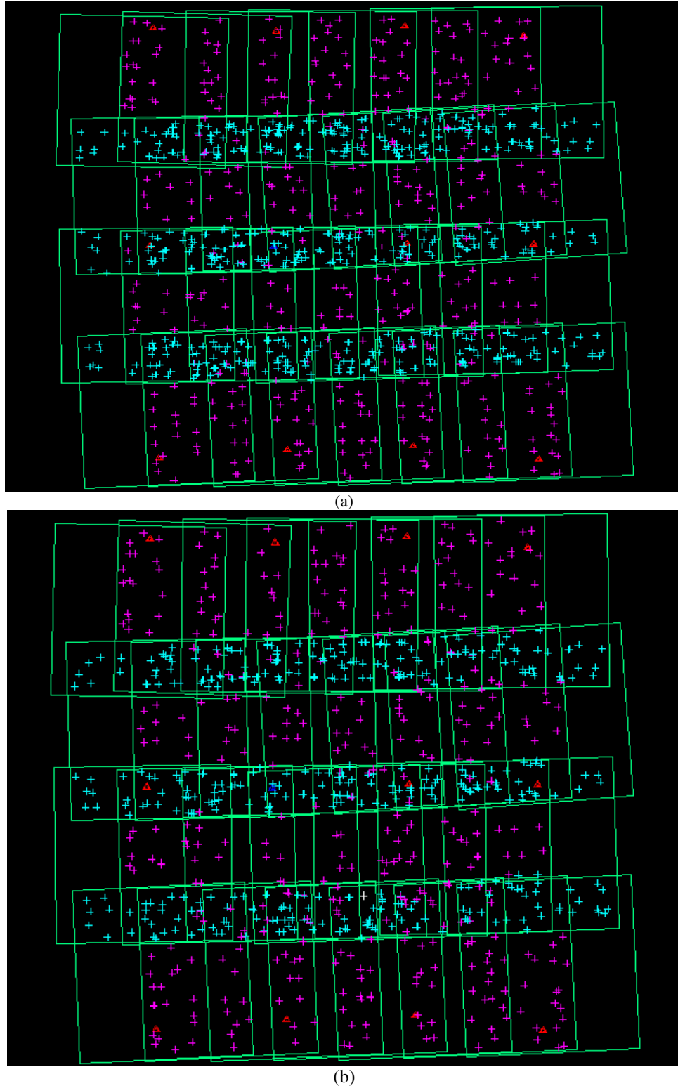
Figure 6. Distribution of Automatically Generated Tie Points Before and After Removal of Shadow Points (+ represents pass points within strips, + denotes tie points cross strips) (a) before removal of shadow points, (b) after removal of shadow points
