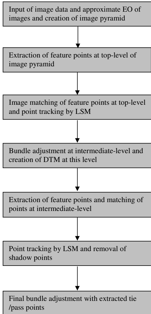
Figure 1. Automatic Generation of Tie/Pass Points in Z/I Imaging's ISAT
