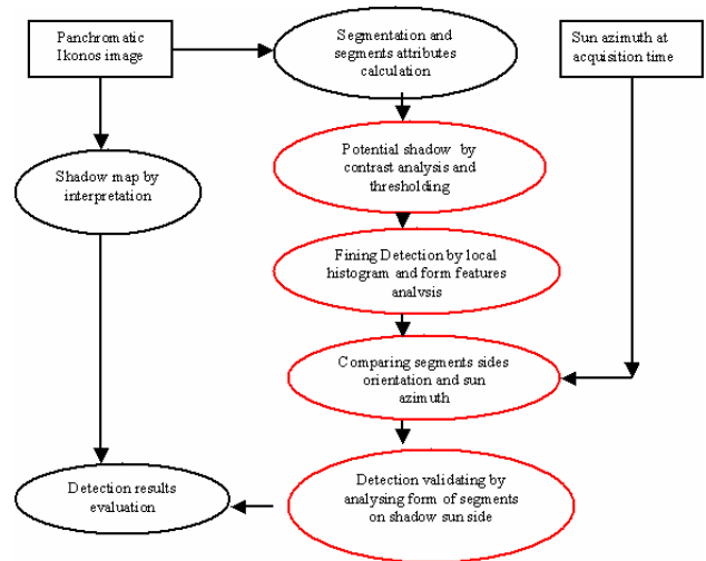
Figure 1: Diagram for the shadow detection
