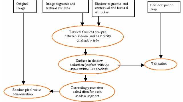
Figure 2: Diagram for information recovery and de-shadowing.
