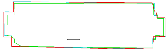
Figure 12. The boundaries of Building1: Light Blue one was generated by the real 1 meter Lidar data; Green one was generated by the 3 meter Lidar data; and Red one was generated by the densified 1 meter Lidar points. The bar in the middle of the drawing represents 10 meter distance.
