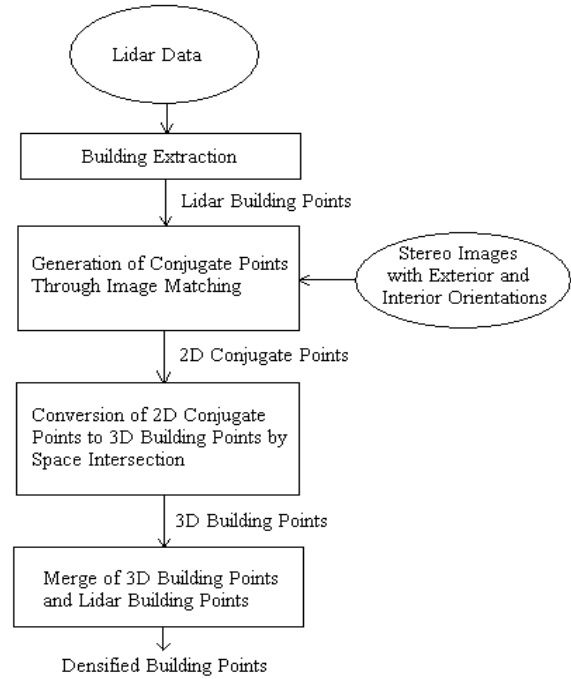
Figure 1. The processes and data flow of the LPDS.
