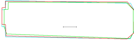
Figure 13. The boundaries of Building2: Light Blue one was generated by the real 1 meter Lidar data; Green one was generated by the 3 meter Lidar data; and Red one was generated by the densified 1 meter Lidar points. The bar in the middle of the drawing represents 10 meter distance.
