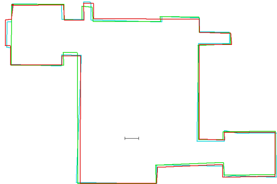
Figure 14. The boundaries of Building3: Light Blue one was generated by the real 1 meter Lidar data; Green one was generated by the 3 meter Lidar data; and Red one was generated by the densified 1 meter Lidar points. The bar in the middle of the drawing represents 10 meter distance.
