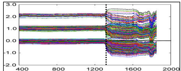
Figure 5: Values of n components of e along the iterations.
