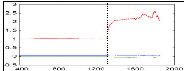
Figure 4: Values of \theta_0 (red), \theta_1 (blue), \theta_2 (green).
