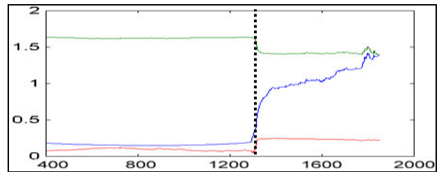
Figure 3: Values of \hat{\sigma}_{\text{dataset}} (green), \hat{\sigma}_{\text{subset}} (blue), \hat{\rho} (red).
