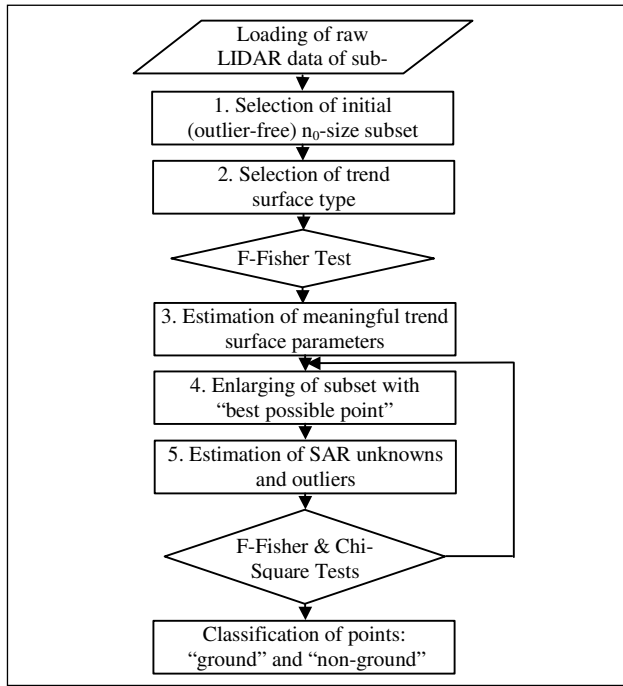
Figure 1: Work-flow of the SFS filtering algorithm.
