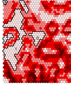
Figure 7: Five clusters detected from Umatrix of the SOM
