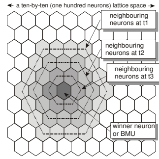
Figure 2: The characteristics of a 10x10 SOM ( t_1 < t_2 < t_3 with h_{ci}(t) in equation 3)
