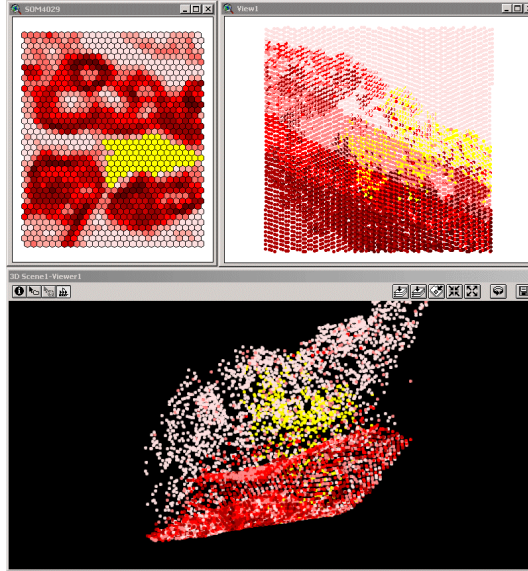
Figure 4: An interface with three connected visual components: SOM, 2D view and 3D scene of a point cloud
