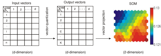
Figure 1: Illustration of SOM principle
