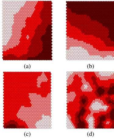
Figure 6: Component visualizations of the SOM: (a) x coordinate, (b) y coordinate, (c) z coordinate, and (d) intensity
