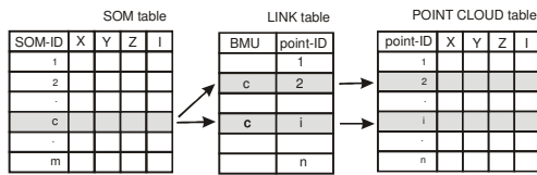
Figure 3: Linkage between a SOM and point cloud
