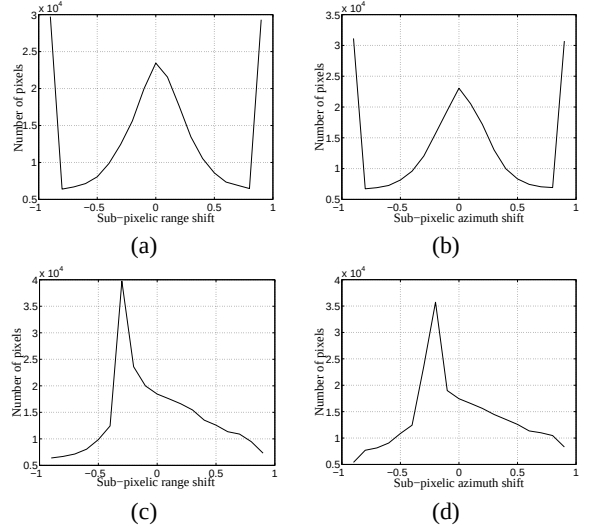
Fig. 1. Examples of histograms of the azimuth and range shifts computed with the new algorithms from (a) & (b) the Mustang and (c) & (d) Orgeval tandem pairs.
