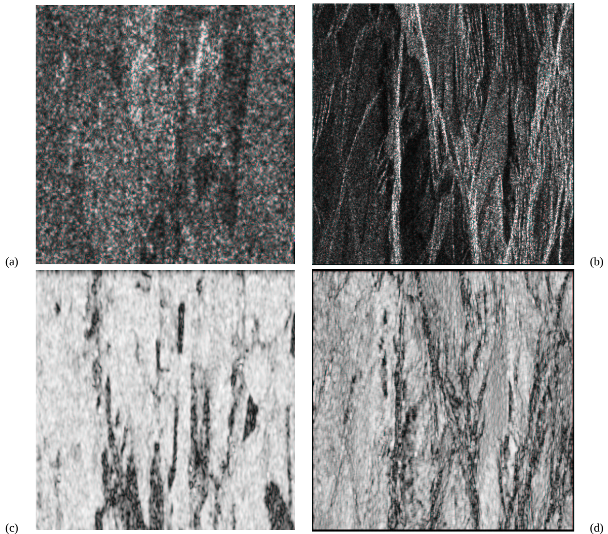
Fig. 2. SLC ERS interferometric pair tandem of (a) Orgeval and (b) Mustang and their corresponding coherence image (c) and (d). The coherence maps were computed with the ISAR software.
