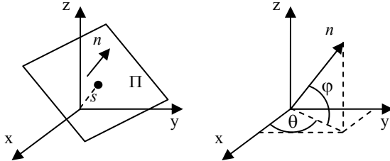
Figure 1. Parameterization of planes in \mathbb{R}^3 .
