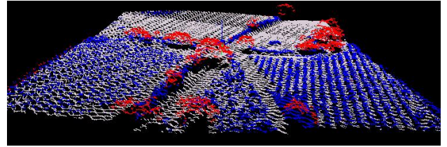
Figure 5: 3D view of a classified laser landscape over the area of Roujan, France. White, blue and red points are respectively ground, low non-ground and non-ground laser points.
