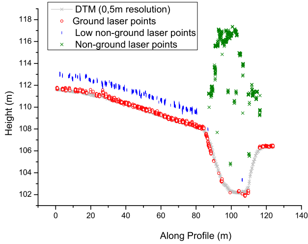
Figure 6: profile of both the final DTM (in gray) and the classified laser points over an other location of the Roujan data set. red circles, vertical blue dashes and green crux are respectively ground, low non-ground and non-ground laser points.
