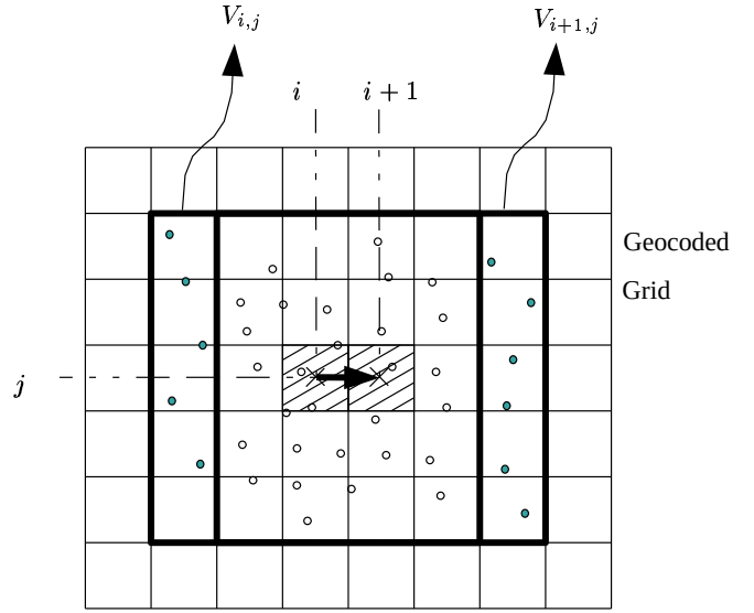
Figure 3: V_{i,j} represents the neighborhood at grid cell (i, j) whereas V_{i+1,j} is the next neighborhood extraction following the propagation route. Empty circles are common laser points, which will be consecutively processed. The ground estimation is performed onto \mathcal{S}_{in}(i, j) , \mathcal{S}_{in}(i + 1, j) \dots using points classified as ground within a laser neighborhood V_{i,j} , V_{i+1,j} \dots
