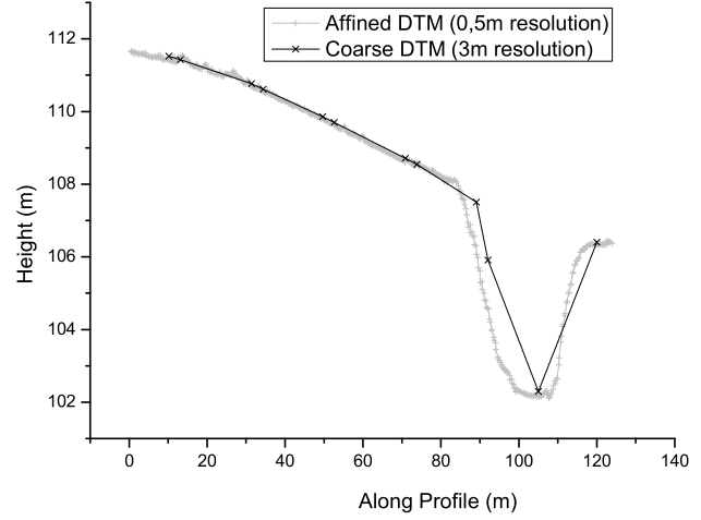
Figure 7: Black line depicts \mathcal{S}_{in} (DTM after the classification process). Gray line is the final DTM at the top end of the process.
