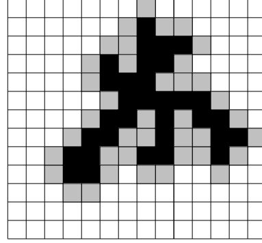
Figure 1: Aspect of the propagation on a geocoded grid. Black cells have already been visited whereas gray ones are potential candidates
