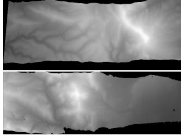
Figure 8: Resulting 0.5 m resolution DTM of the classification of a mountainous area near Montmirail, South of France. These two pictures represent the same laser strip split up for the presentation concerns. It is a 16 km long and 2.3 km wide strip.
