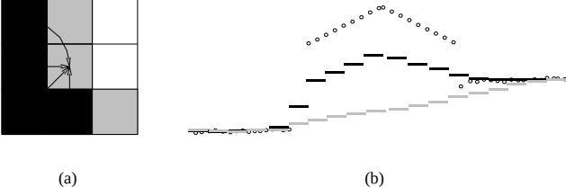
Figure 2: (a) Black cells have already been visited whereas gray ones are potential candidates for propagating (see Figure 1). \hat{Z}_{ground\ local} is calculated by averaging elevation over black cells. (b) Illustration of the linear correction. Empty circles are laser points. Black dash lines are the estimated local ground \hat{Z}_{ground\ local} without linear correction whereas gray dash lines are the estimated local ground \hat{Z}_{ground\ local} after linear correction
