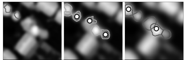
Figure 6: Valid hypotheses for trees in different scale levels, depicted are the borderlines in different grey values. Best hypotheses are marked with a white circle.
