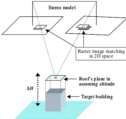
Figure 8. Process flow of indirect comparison method
