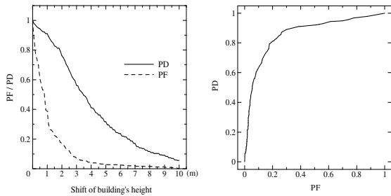
Figure 14. Change detection ability by 3D image matching method (1995 - 2003)
