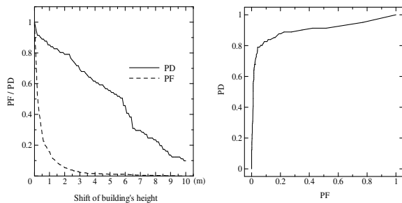
Figure 15. Change detection ability by 3D image matching method (1998 - 2003)
