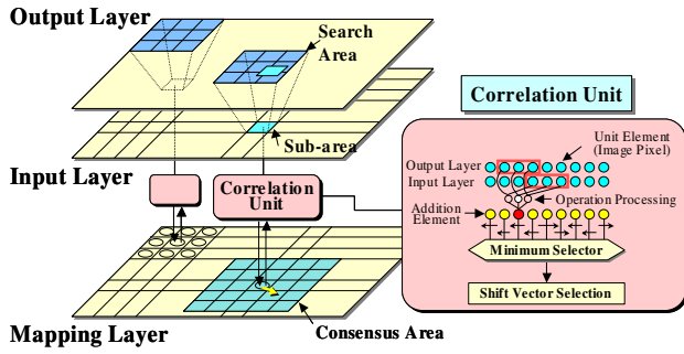
Figure 5. Conceptual diagram for adaptive nonlinear mapping
