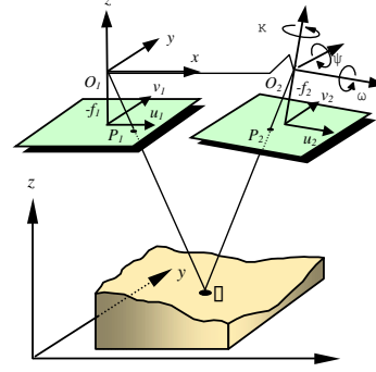
Figure 4. Coordinate system in a stereo model
