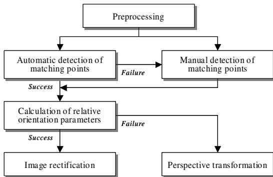
Figure 3. Process flow for formation of imaginary stereo model
