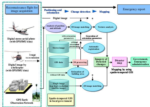
Figure 1. Urgent correspondence system for a huge earthquake occurrence
