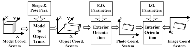
Figure 7. The coordinate systems involved with LSMIF.
