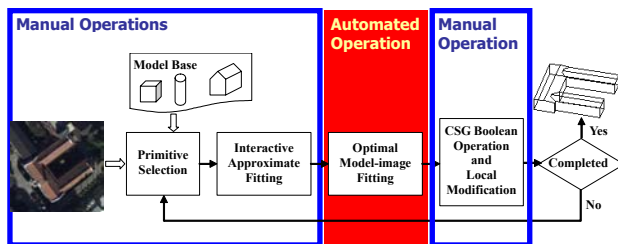
Figure 1. The proposed semi-automated strategy for model-based building extraction.
