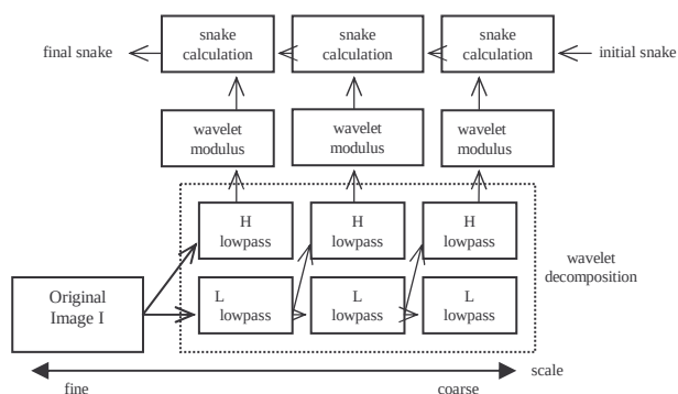
Figure 1. Flow chart of the wavelet-based active contour model
