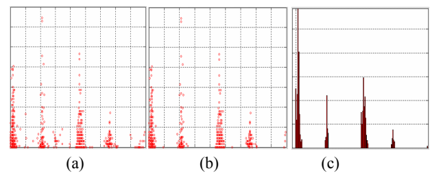
Figure 3. Angle – length relationship for line segments. (a) Angle and length for all line segments. (b) Result after 90-degree filtering. (c) Histogram after 90-degree filtering and threshold.
