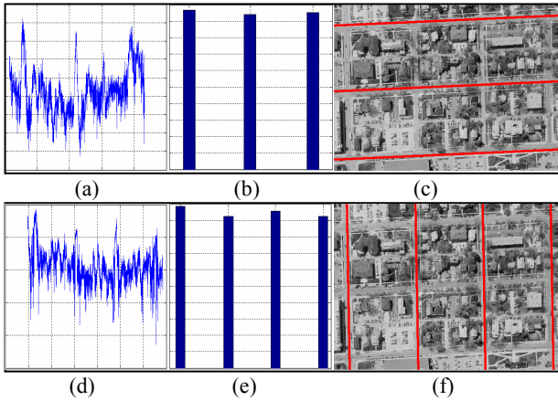
Figure 7. Result of acupuncture method on small example region. (a)~(c) are for \theta_{d1} , and (d)~(f) are for \theta_{d2} . (a) and (d) Free passage measure. (b) and (e) Clustering result. (c) and (f) Detected lines on the road.
