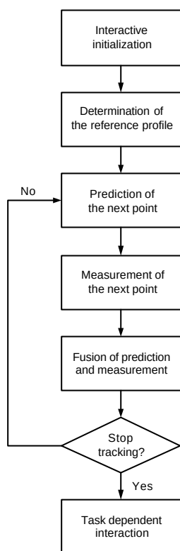
Figure 5. Flow chart of the line following algorithm
