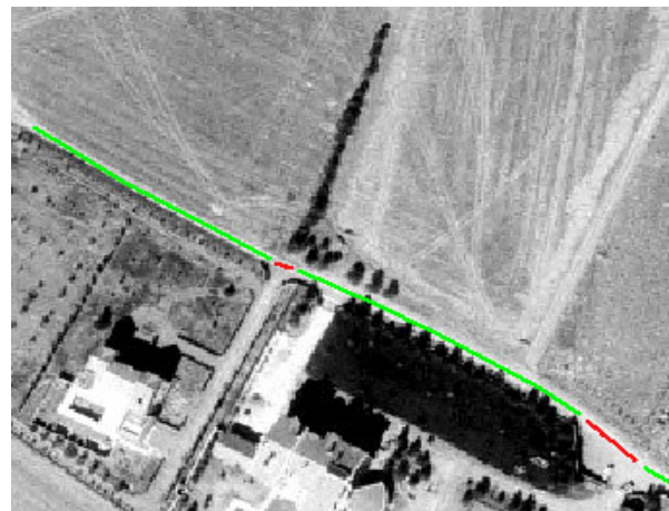
Figure 1. Road tracing by profile matching and Kalman filter
