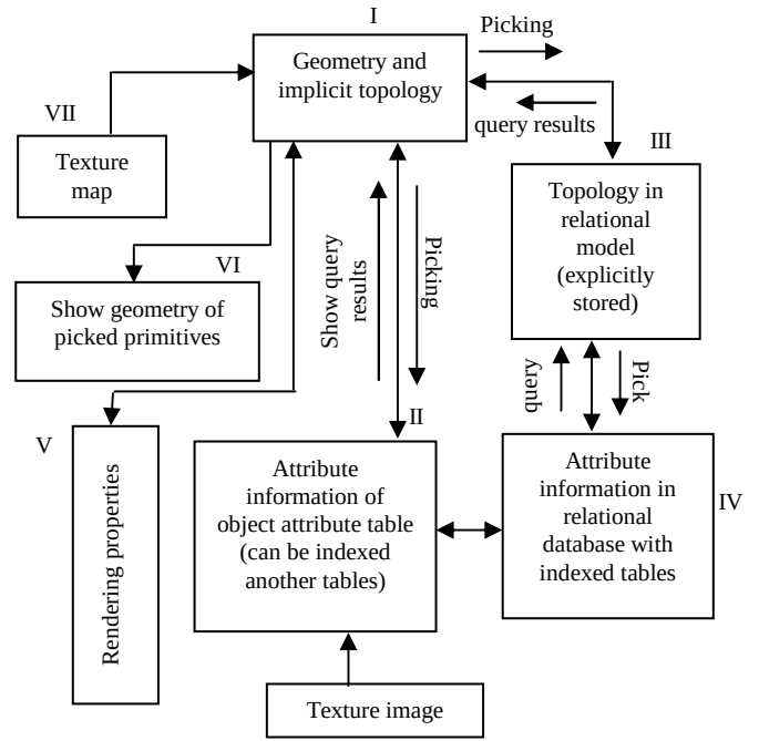
Figure 3. General representation of geometry and topology
