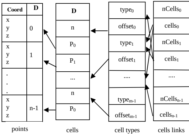
Figure 2. Implicit representation of geometry and topology
