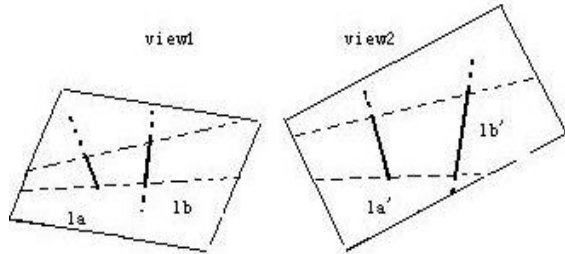
Figure 4: epipolar constraint
