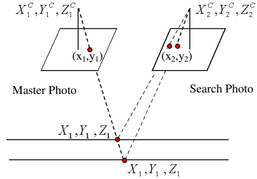
Figure 2. Stereo measurement via monoscopic viewing.
