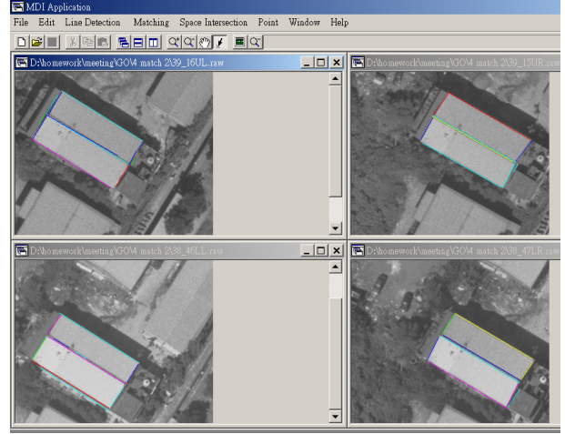
Figure 6. Case 2- Simple gable roof.
