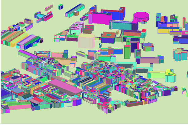
Figure 4. The generated 3D building model based on manual stereo measurement of visible roof-edges.
