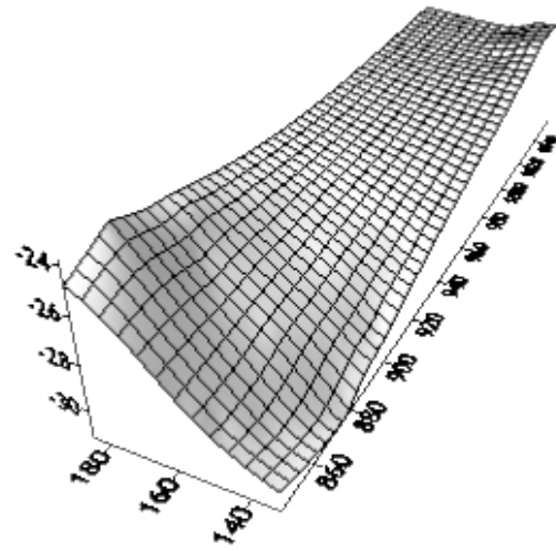
Figure 2b. The three-dimensional surface plot of the deformed steel surface
