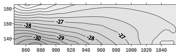
Figure 2a. Contour plot of the deformed steel surface
