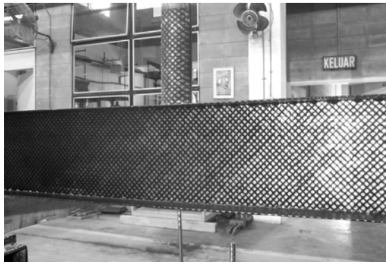
Figure 1 An image of the steel beam tested
