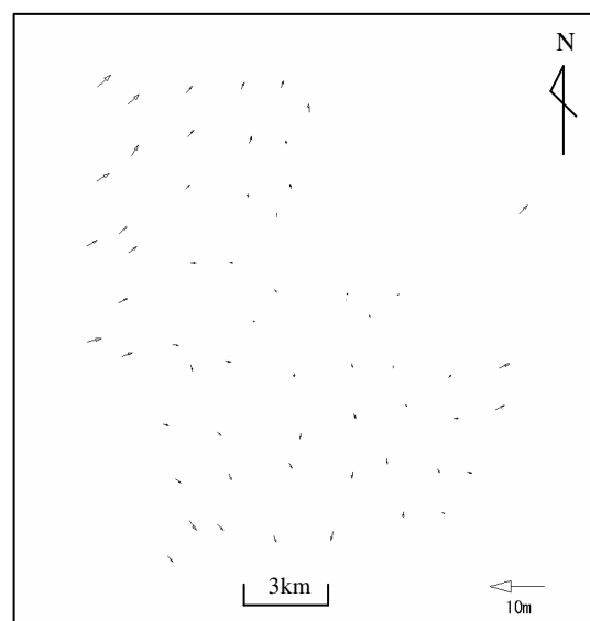
Fig.6 Horizontal component of error vectors (after correction)
