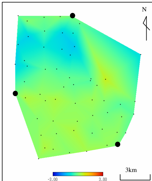
Fig.8 Vertical errors after correction with 3 GCPs taken from coastline (●: GCP)
