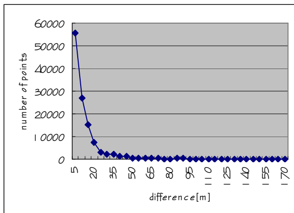
Fig. 14 the comparison between two DSMs
