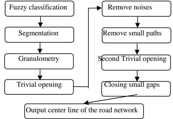
Figure 3. Block diagram used in morphology approach
