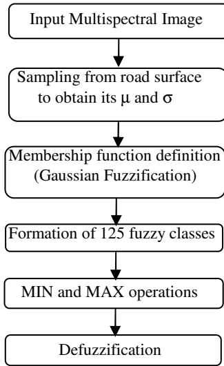
Figure 2. Implementation flowchart in fuzzy step
