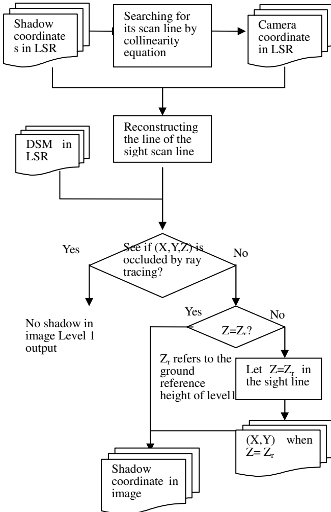
Figure 2 Flow chart of shadow tracing
