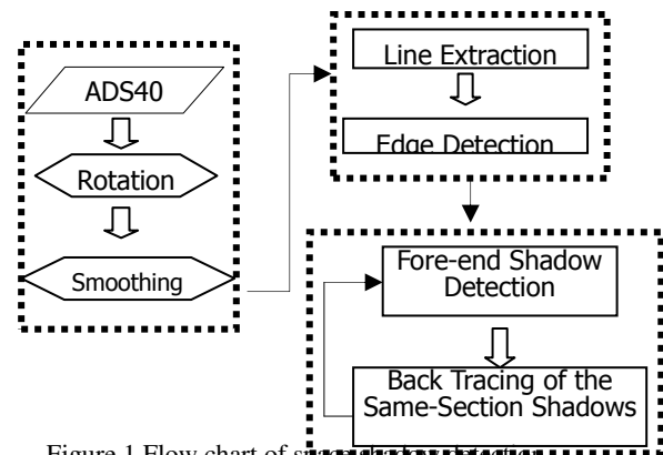
Figure 1 Flow chart of space shadow detection
