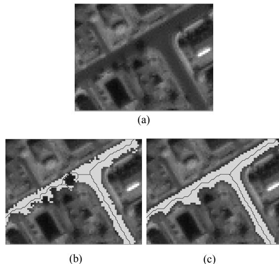
Figure 7. Effect of applying region growing on a smoothed image. (a) original, (b) result of region growing on original, (c) result of region growing on smoothed image
