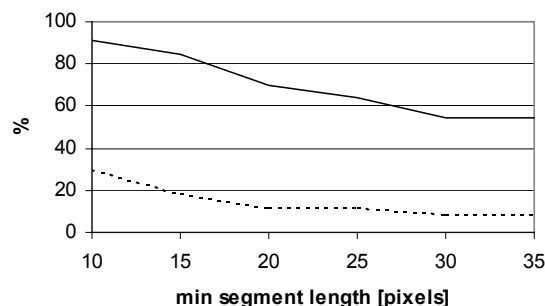
Figure 8. Detection rate versus minimum segment length. Full curve gives true positives. Dashed curve gives false positives.
