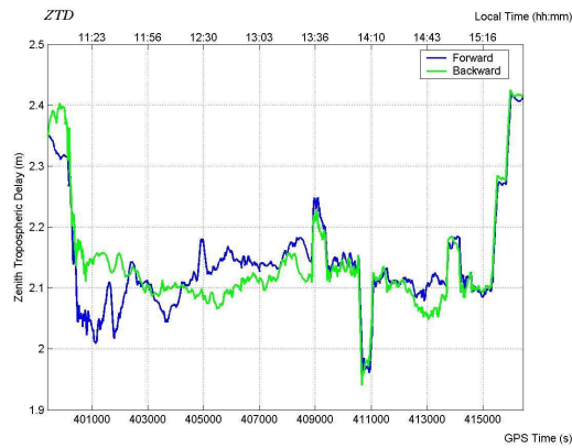
Figure 4: Zenith Tropospheric Delay
