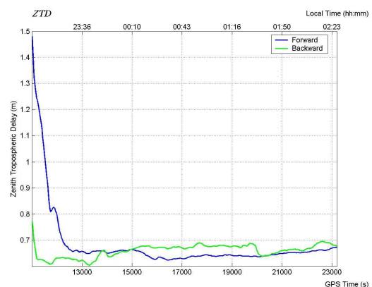
Figure 8: Zenith Tropospheric Delay
