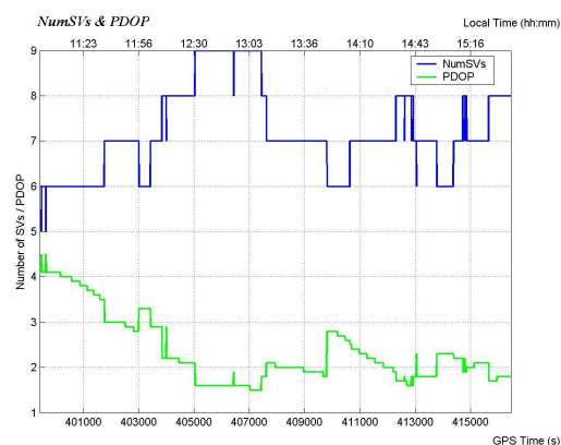
Figure 2: Number of Satellites and PDOP
