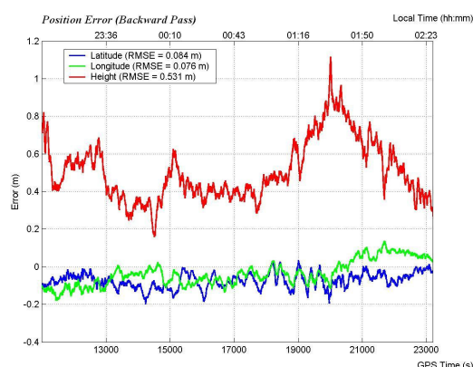
Figure 10: Position Errors between P 3 and the Data Supplier's In-House DGPS Solution
