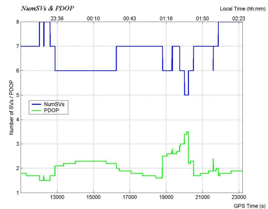
Figure 6: Number of Satellites and PDOP
