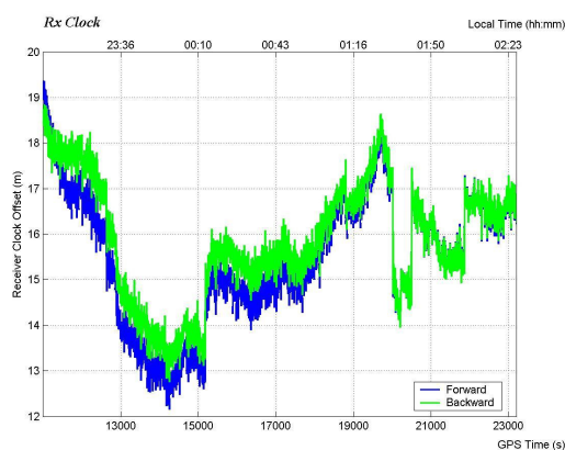
Figure 9: Receiver Clock Error
