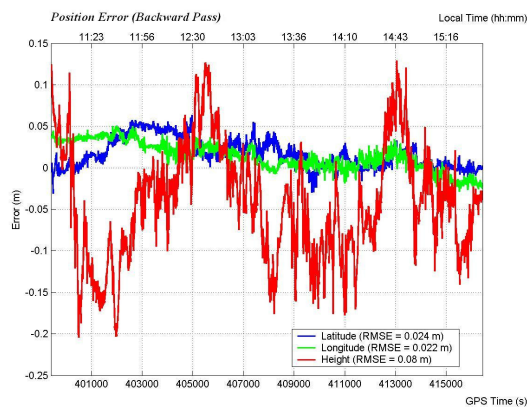
Figure 5: Position Errors between P 3 and JPL's GIPSY/OASIS II Solution
