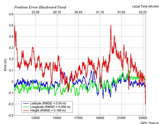
Figure 11: Position Errors between P 3 and JPL's GIPSY OASIS II Solution
