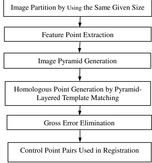
Fig.2 Generation of control points by automatic image matching
