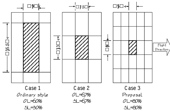
Figure 12. Scope of processing and angle of view of photograph
