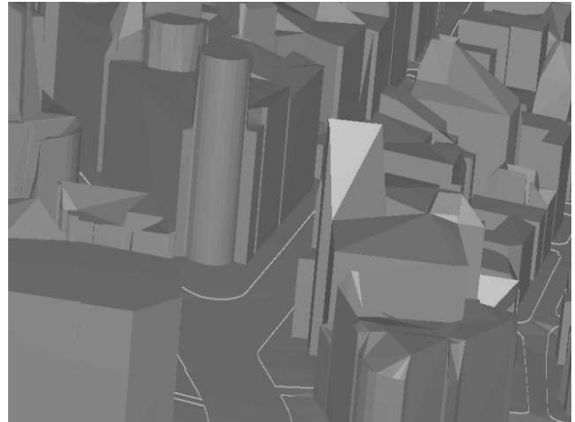
Figure 6. 3-dimensional surface model around High buildings
