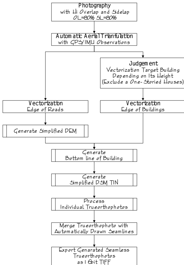
Figure 5. Flowchart of True orthophoto generation method
