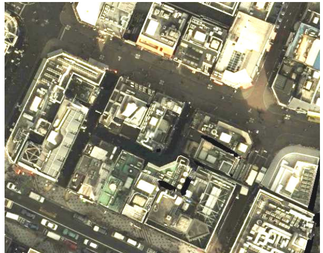
Figure 11. Generated true orthophoto same area as figure 10
