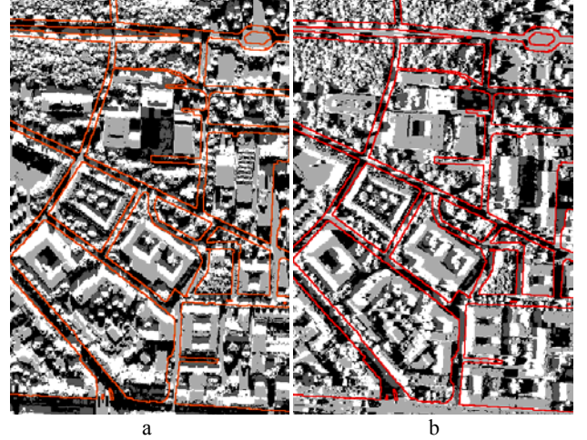
Figure 9. Simulation results for given SAR parameters from Fig 8b. (layover: white, shadow: black, layover+shadow: dark gray, reliable: bright gray). a) illumination from north (top), b) illumination from west (left).
