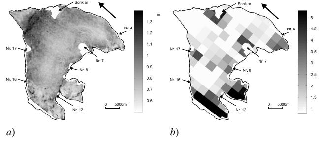
Figure 8: a) Theoretical standard deviations of the estimated DSM [m]. b) Adjusted variance factors for Hall Island. One variance factor is estimated for each of the 14 \times 14 tiles.
