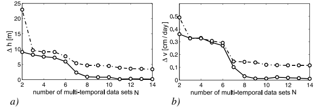
Figure 3: Effect of non-modeled atmospheric effects on the estimated unknowns topography (a) and motion (b) for polar regions.
