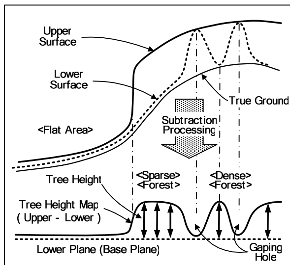
Figure 4. Extraction of Tree Height Map
