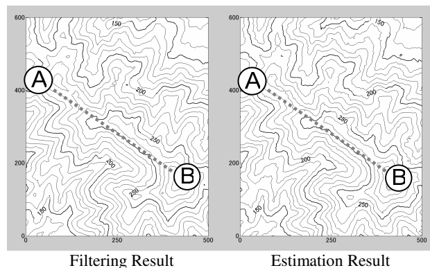
Figure 11. Contour Line Comparison in Shimane (Medium Forest)
