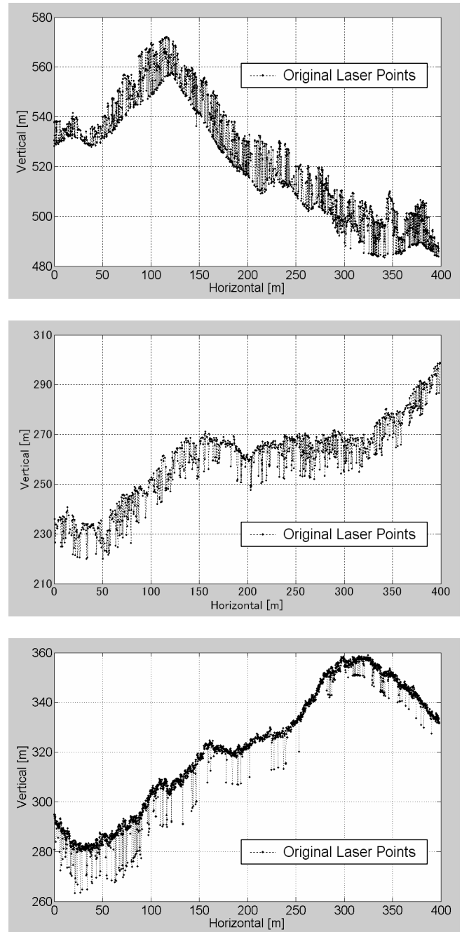
Figure 8. Cross Section of Measurement Data (Upper: Hokkaido / Middle: Shimane / Lower: Wakayama)
