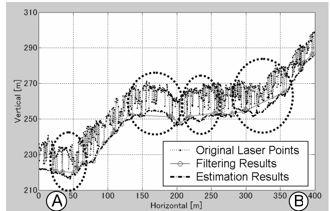
Figure 12. Cross Section in Shimane (Medium Forest)
