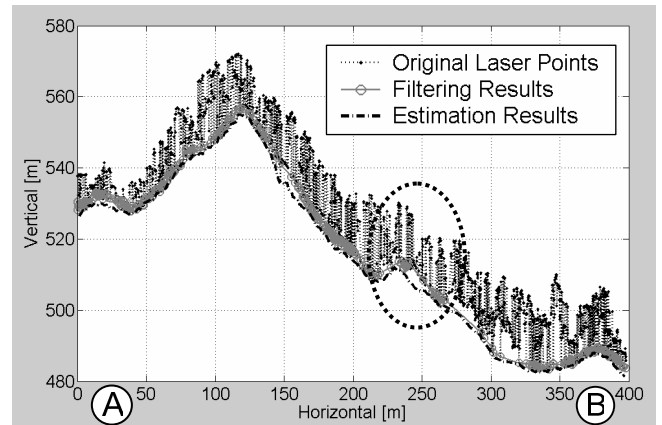
Figure 10. Cross Section in Hokkaido (Sparse Forest)
