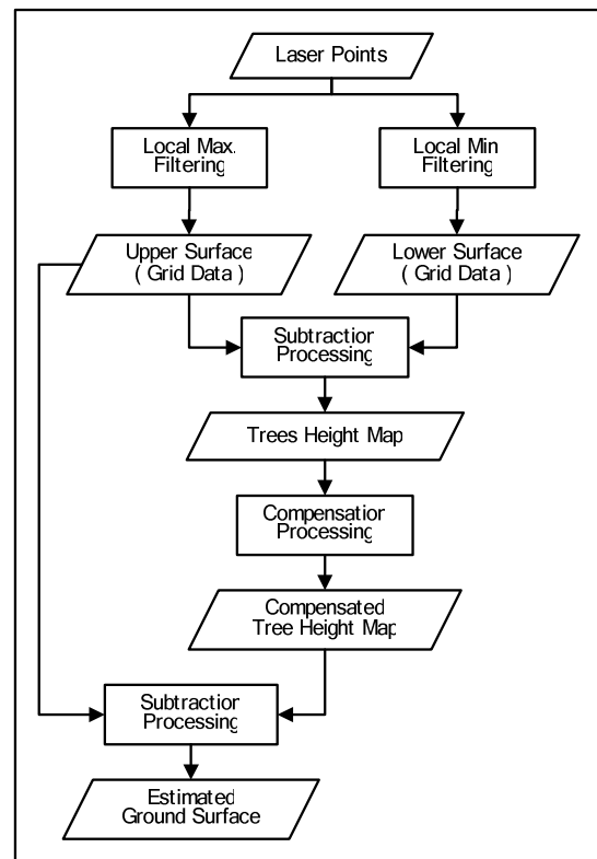
Figure 3. Flow of Proposed Method
