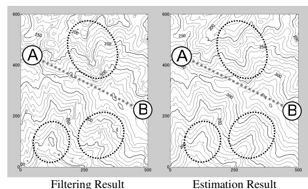
Figure 13. Contour Line Comparison in Wakayama (Dense Forest)
