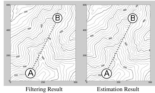
Figure 9. Contour Line Comparison in Hokkaido (Sparse Forest)
