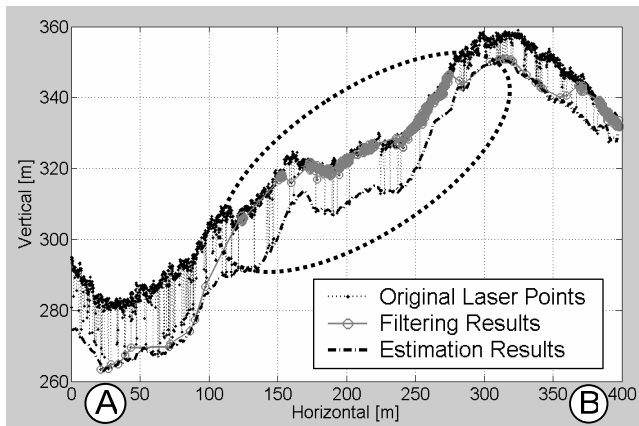
Figure 14. Cross Section in Wakayama (Dense Forest)
