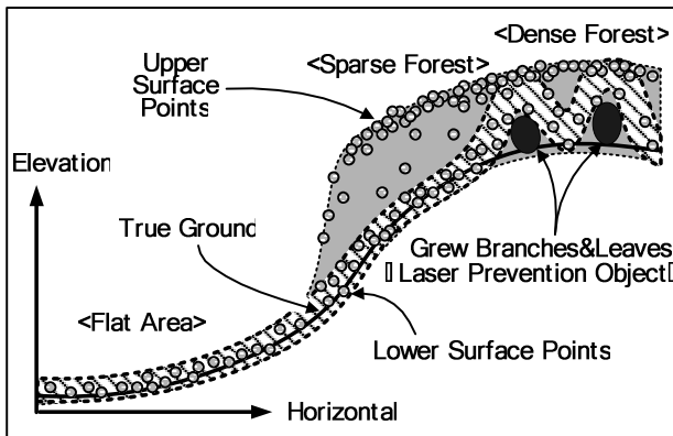
Figure 2. Characteristic of Laser Data in Dense Forest
