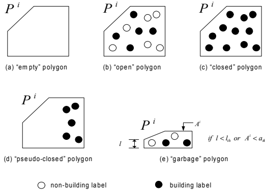
Figure 8. Polygon classification
