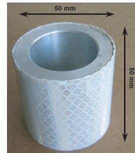
Figure 2: Reflector target
