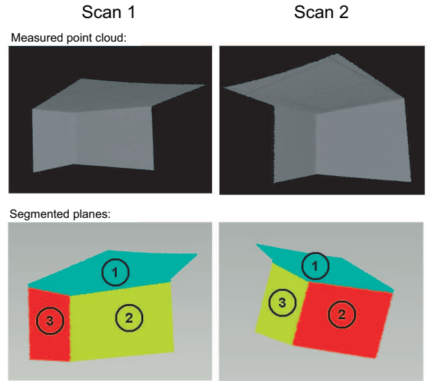
Figure 6: Test data
